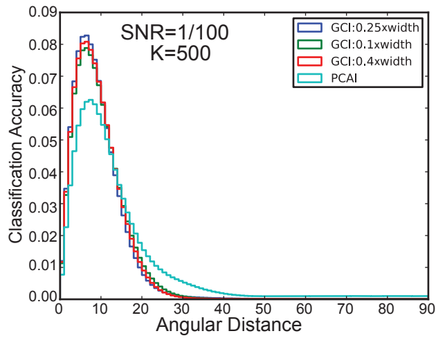
Radius=0.1xwidth
