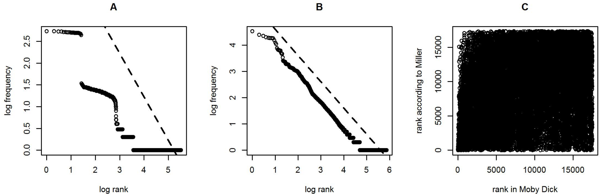
Simulation of Miller's proposal. A: predicted frequency by rank in double-log space with uniform character probability. B: using differential character probability (as determined by Moby Dick ). Dashed lines show ideal Zipfian distribution. C: rank of words in Moby Dick against their rank as predicted by Miller.
