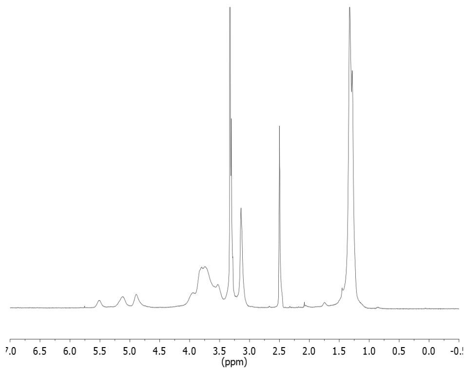
Figure S1. ^1\text{H} NMR spectrum of acetalated dextran (Ac-Dex) in DMSO
