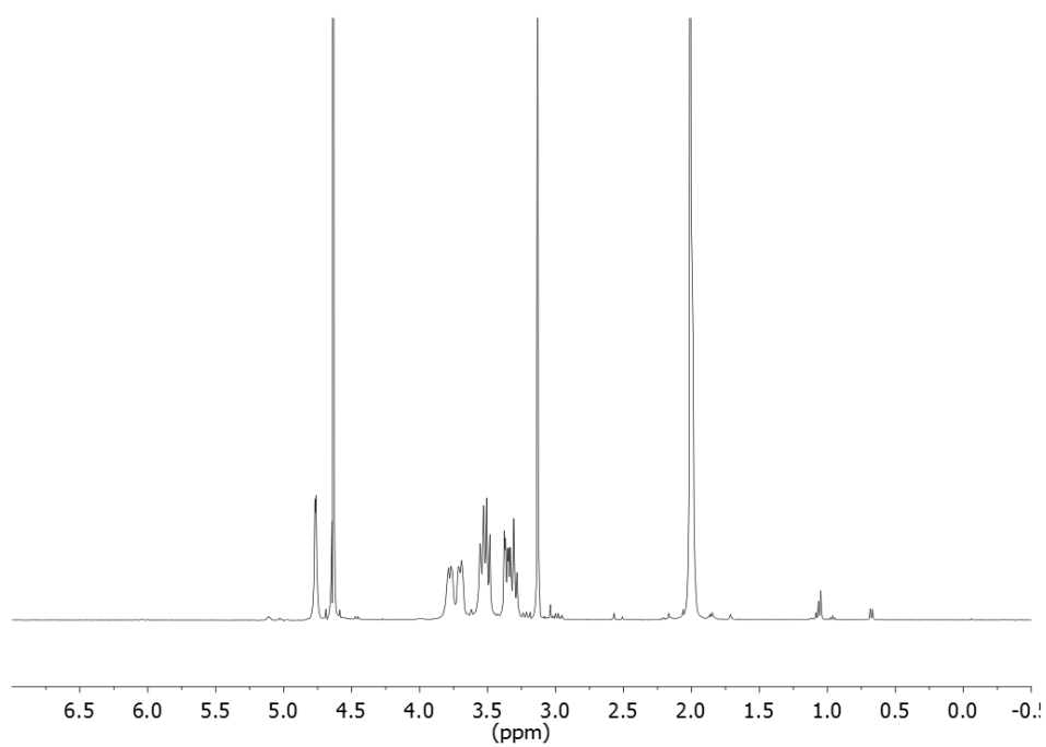
Figure S2. ^1\text{H} NMR spectrum obtained after deprotection of Ac-Dex in dilute DCl solution.
