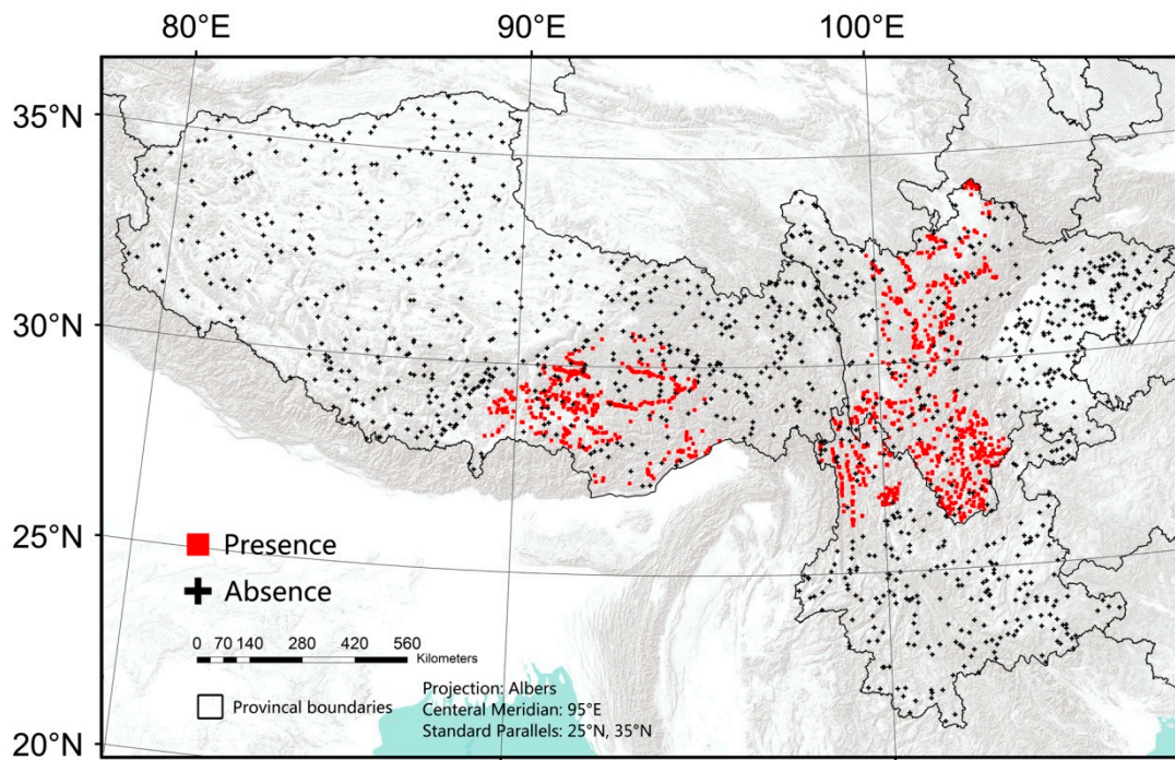
Figure S1. Example of a set of training samples (A total of 1000 training subsets were generated randomly in the bootstrapping logistic regression analyses.)
