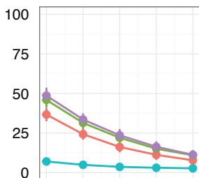
ECFP6
