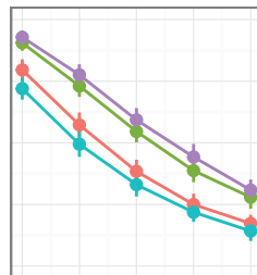
ECFP4
