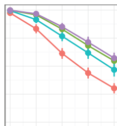
FCFP4
