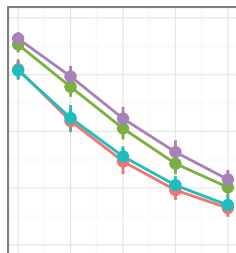
ECFP0
