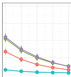
FCFP0
