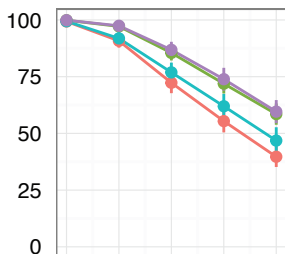
FCFP6
