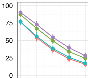
E-state
