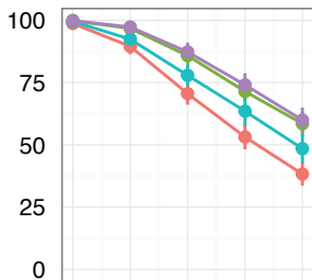
MACCS
