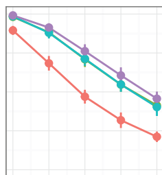
FCFP2
