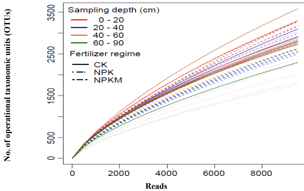
Figure S1. Rarefaction curves (cutoff 0.03) of the soil microbiota within the whole soil profile (0-90 cm) under different long-term fertilizer treatments.
