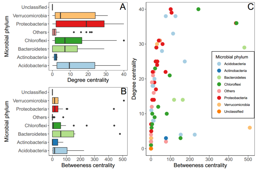
Figure S6. The degree and betweenness centrality of correlation network of subsoils (20-90 cm).
