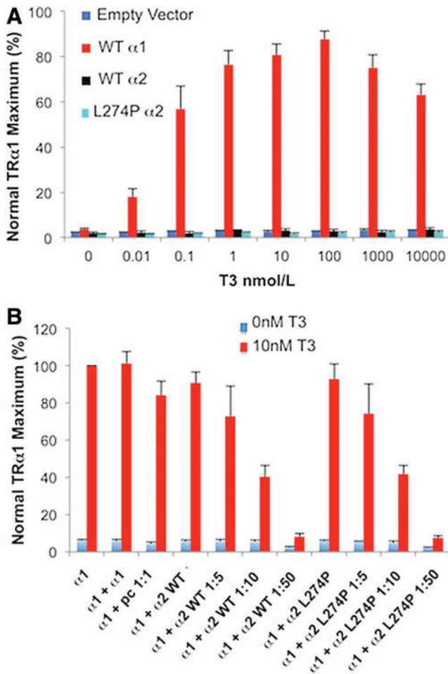
SUPPLEMENTARY FIG. S4. JEG-3 cells were transfected with empty, WT TR \alpha 1 or TR \alpha 2, or L274P mutant TR \alpha 2 expression vectors together with a thyroid hormone responsive reporter gene assaying T3-dependent activation. Dominant negative inhibition by WT or L274P mutant TR \alpha 2 was tested in JEG-3 cells cotransfected with reporter gene and combinations of expression vectors as indicated.
