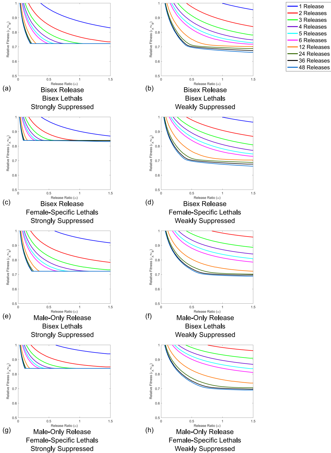
Figure S1: Different multiple release strategies and genetic systems produce different conditions for transgene introgression. Here each panel represents a more detailed view of the low release ratio regions of Figure 6 in the main text. Each line represents the threshold above which introgression of transgenes into a population is achieved with colours representing different numbers of releases. Details of the scenario considered in each panel are given in the respective labels. Single male-only release of weakly suppressed lethals cannot give introgression even for very large release ratios, hence the omission of a single release threshold line in panels (f) and (h).
