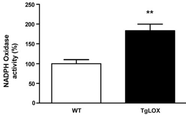
SUPPLEMENTARY FIG. S5. NADPH oxidase activity is induced in vascular smooth muscle cells (VSMC) from LOX transgenic mice. NADPH oxidase activity in VSMC isolated from WT or TgLOX mice. Results are shown as mean \pm SEM ( n=7 ; ** p<0.01 vs. WT).
