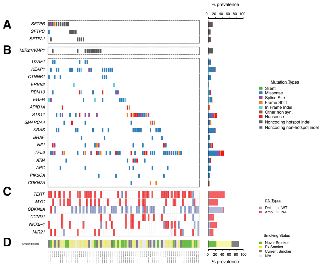
Lung adenocarcinoma WGS cases
