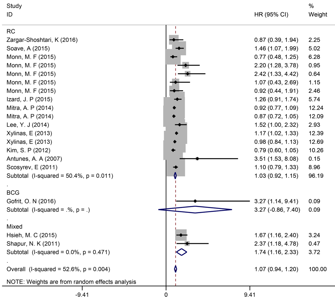
Supplementary Figure 1: Subgroup analysis of different treatments with HVs.
