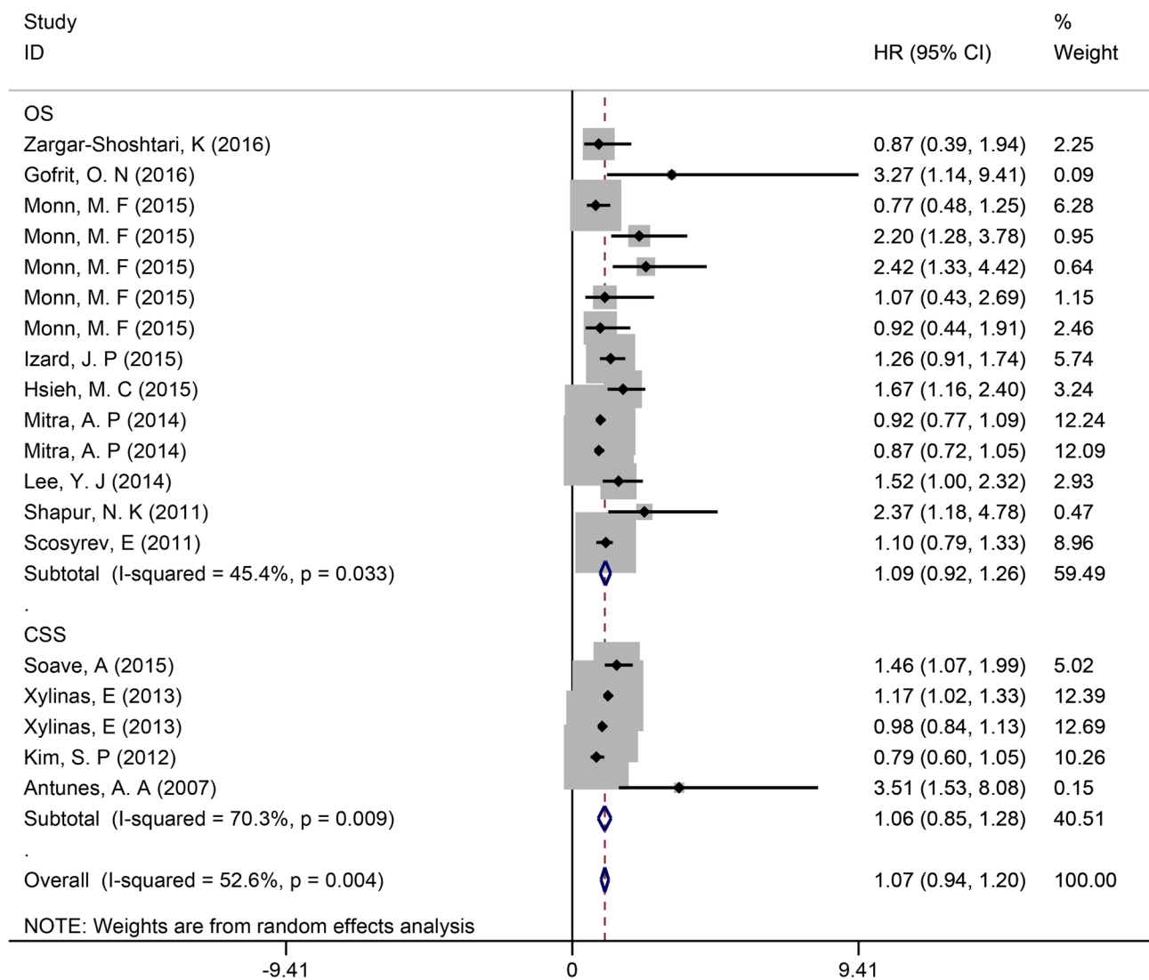
Supplementary Figure 2: Subgroup analysis of different endpoints with HVs.
