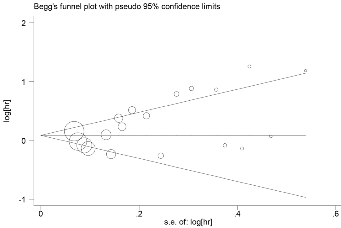
Supplementary Figure 3: Funnel plots of overall analysis.
