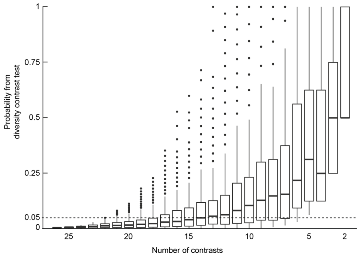
Fig. S3. The probability of the diversity contrast test with declining numbers of contrasts used. The data are the distribution of P values from 1000 random samples taken from the full data set of 25 contrasts.
