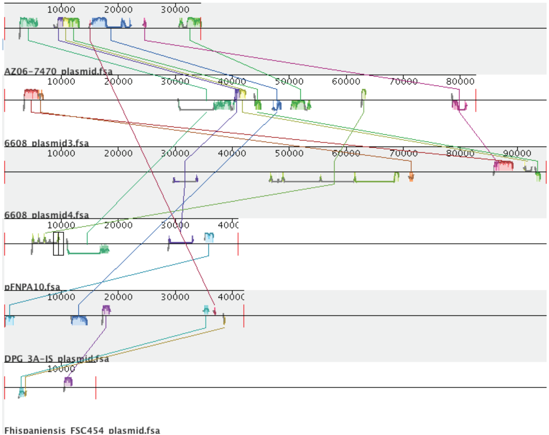
Figure S2. Progressive Mauve alignment of the AZ06-7470 plasmid with TX07-6608 plasmids 3 and 4, pFNPA10 from F. novicida -like strain PA10-7858, the DPG_3A-IS plasmid and the pFSC454 plasmid. The different regions of similarity are shown in different colors.
