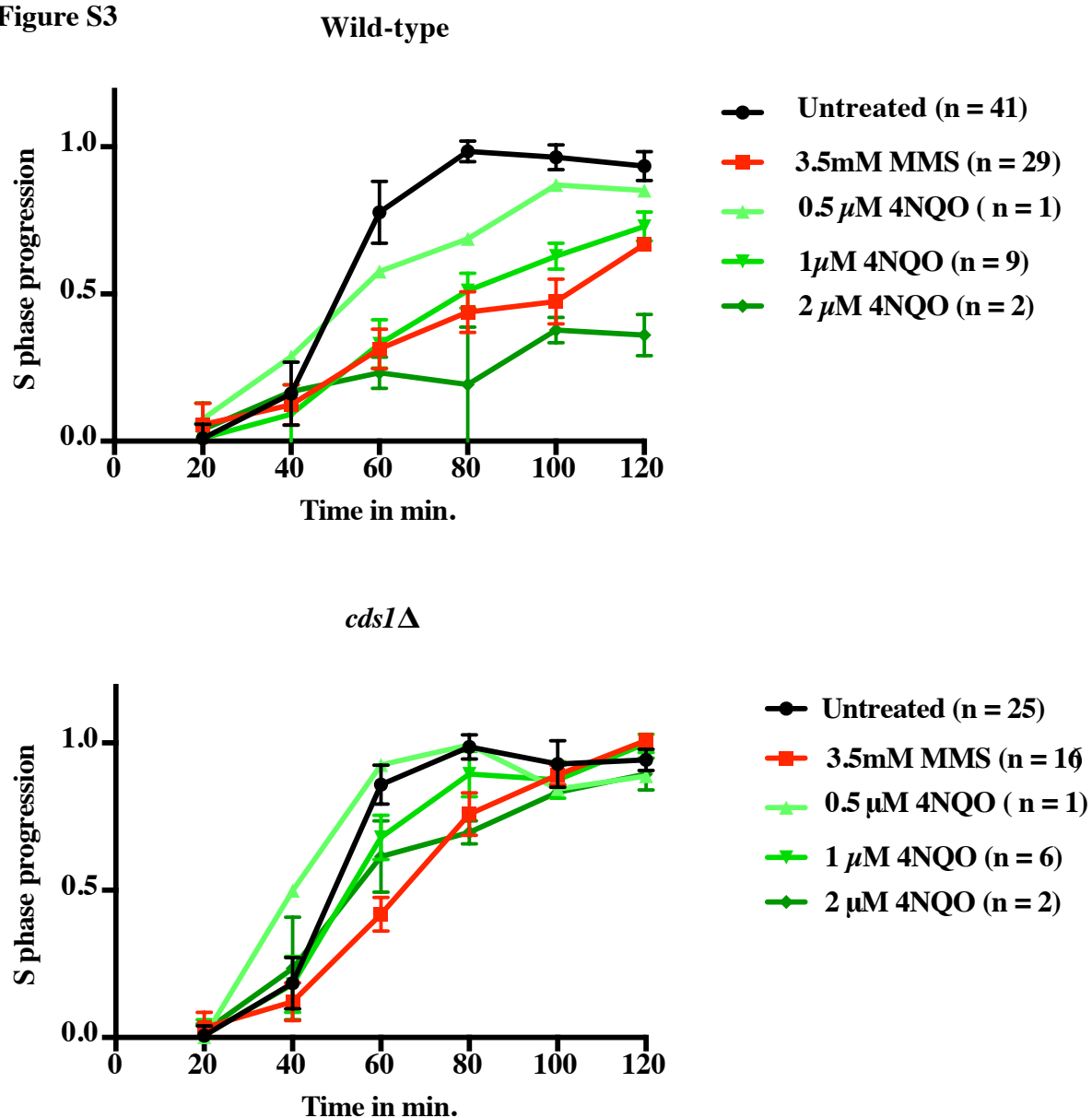
Figure S3: Titration of 4NQO. Wild-type (ySF940) and cds1Δ (yFS941) cells were synchronized and released into S phase with 3.5 mM MMS, 0.5 \mu M, 1 \mu M, 2 \mu M 4NQO or left untreated. S-phase progression was monitored by taking samples every 20 minutes for flow cytometry.
