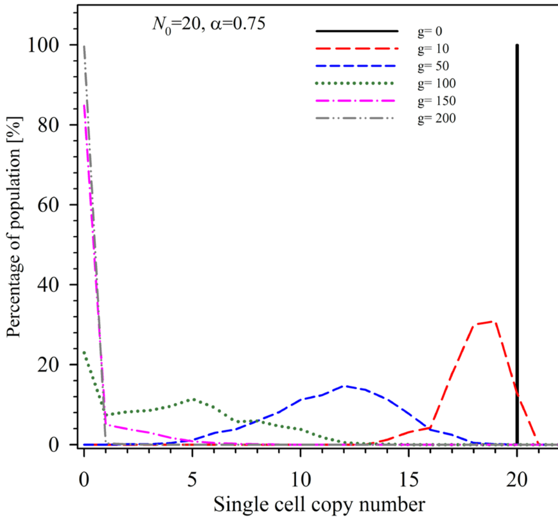
Figure S3. Distribution of PCN in bacterial population after 0, 10, 50, 100, 150 and 200 generations. Initial PCN distribution is derived from equation (9), and N_0=20 and \alpha=0.75 values were adopted.
