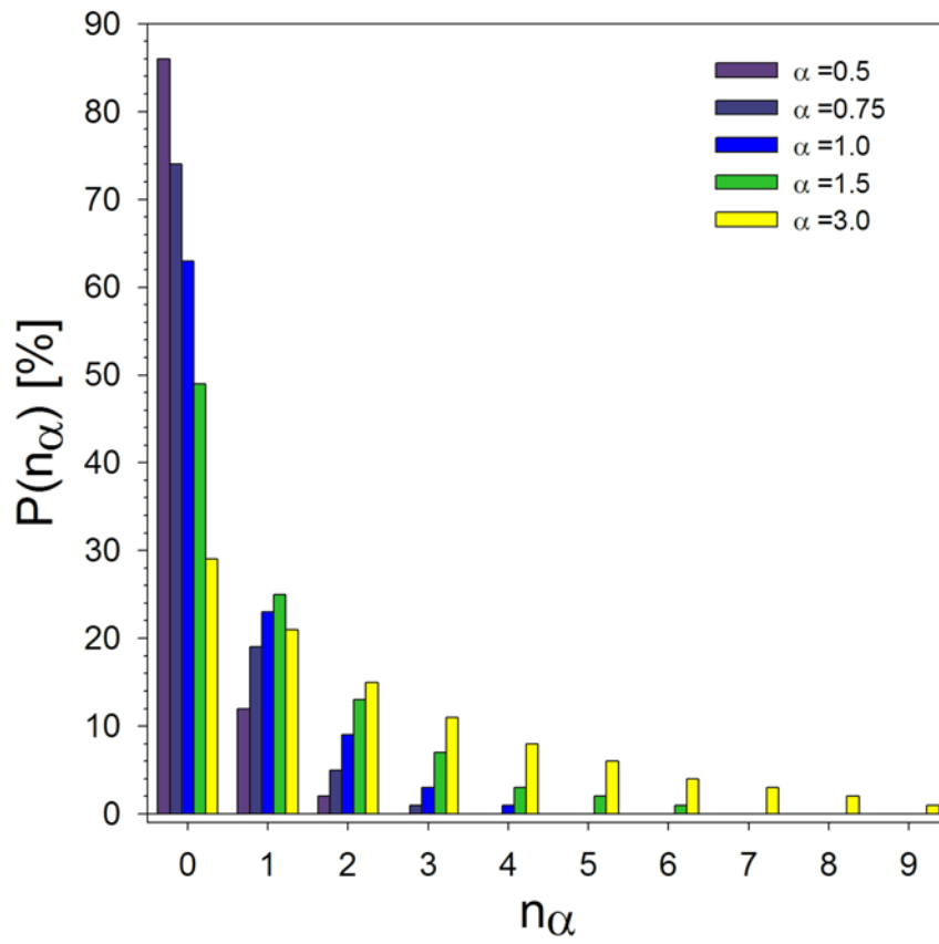
Figure S6. Probability distribution of replication-defective plasmid units ( n_\alpha ) calculated for different values of the \alpha parameter.
