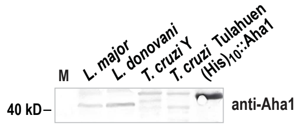
Fig. S1 Anti-Aha1 antibody testing. (His) 10 ::Aha1 was used to raise antibodies in a chicken. Western blot analysis showed that Aha1 antibodies recognise the natural protein in the lysates of L. major , L. donovani , the recombinant protein (His) 10 ::Aha1, but not the orthologues in T. cruzi Y and T. cruzi Tulahuen lysates. Positions of size markers [kD] are shown on the left.
