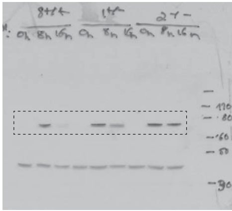
Figure 3D_IE1
