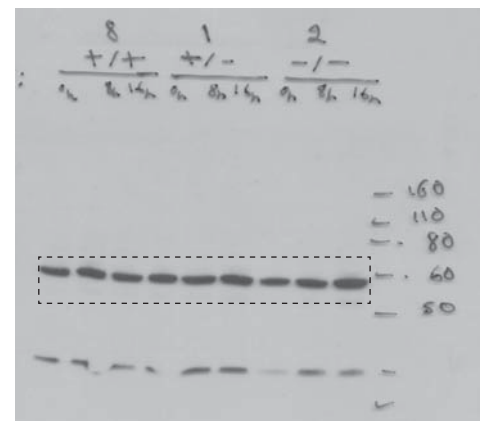
Figure 3D_ZBP1 (Zippy-1)
