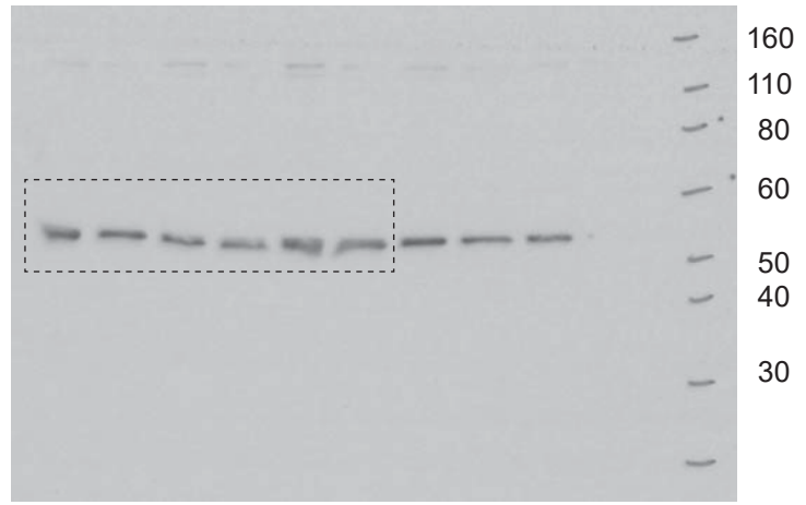
Figure 3A_RIPK3
