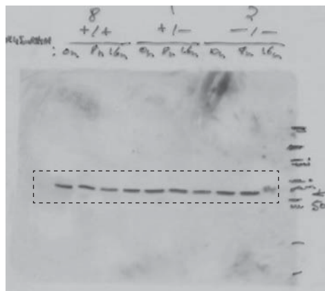
Figure 3D_ZBP1 MLKL
