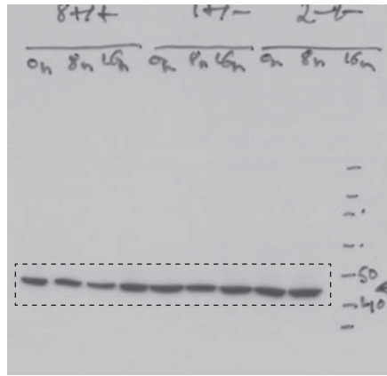
Figure 3D_ACTB
