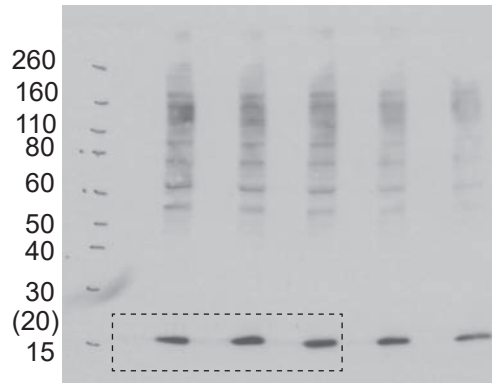
Figure 3A_ISG15
