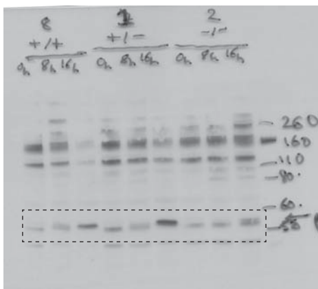
Figure 3D_P-MLKL
