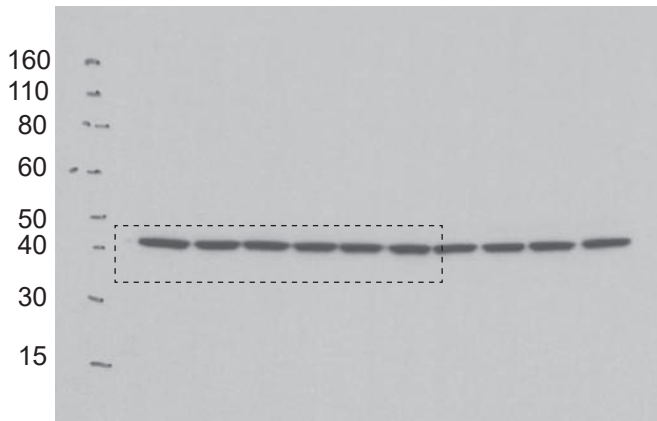
Figure 3A_ACTB
