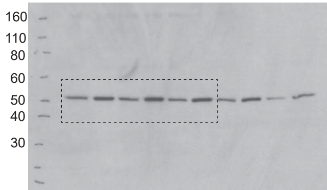
Figure 3A_MLKL
