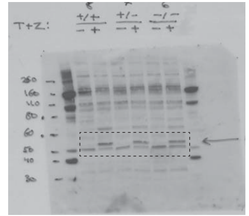
Figure 3E_P-MLKL
