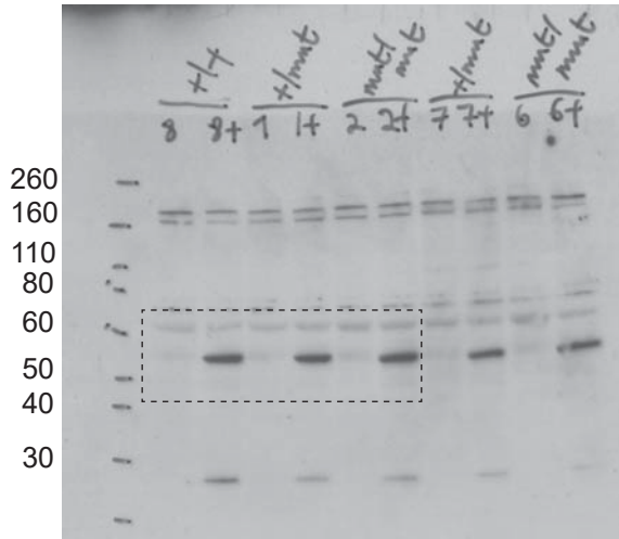
Figure 3A_ZBP1 (Zippy-1)
