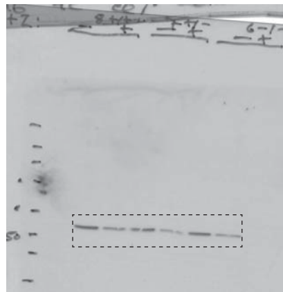
Figure 3E_MLKL
