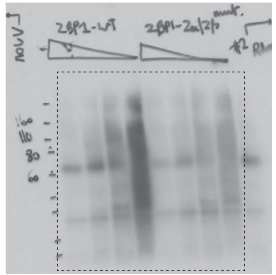
Figure 6D_ autoradiogram
