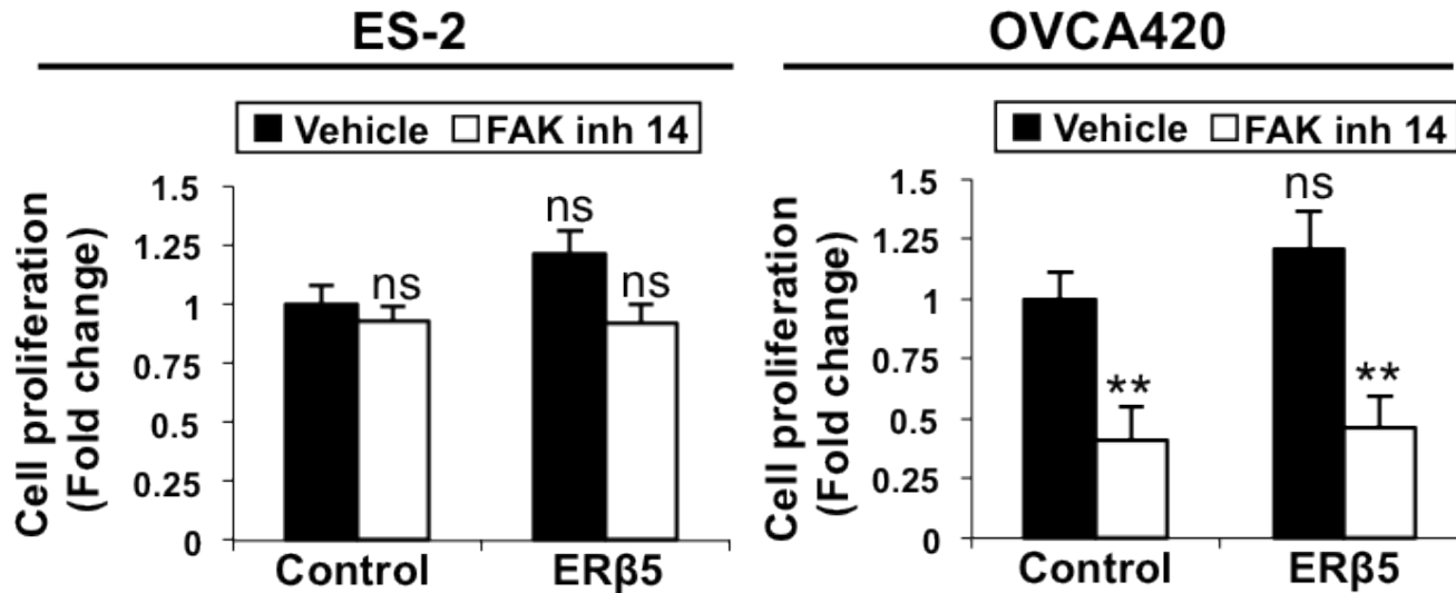
Figure S4. XTT assay revealed lack of significant proliferation effect on day 5 in ES-2 and OVCA420 cells stably transfected with ER \beta 5 as compared to control cells, whereas FAK inh 14 could inhibit OVCA420 basal cell proliferation on day 5. ns, not significant; **, P < 0.005 .
