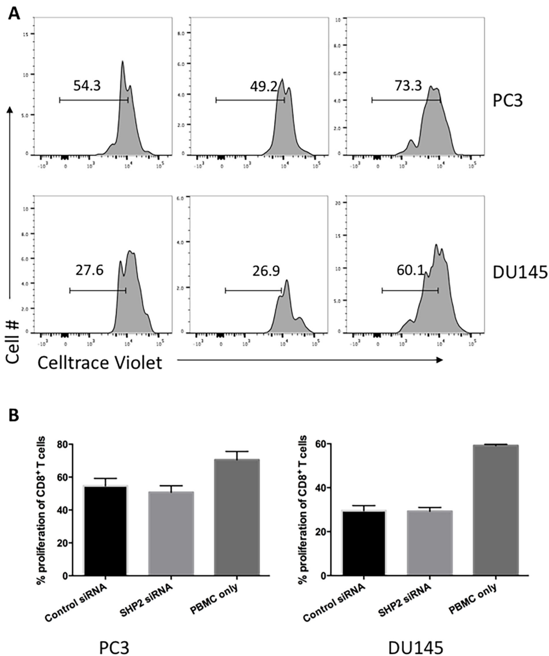
Supplementary Figure 1: SHP2 depletion of PCa cells did not affect CD8 T cell proliferation. (A) Representative flow histograms of CD8 T cells proliferation are shown. (B) Bar graphs represent mean \pm SD from duplicate samples in three independent experiments.
