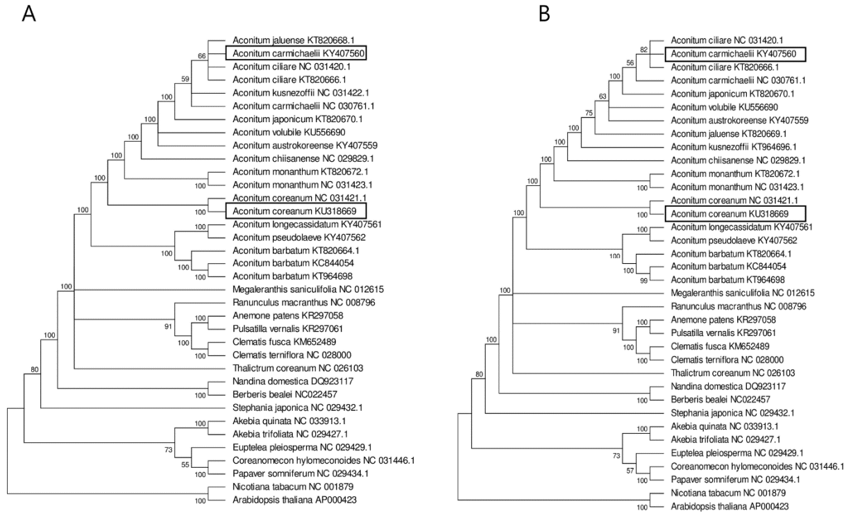
S2 Fig. Molecular phylogenetic tree of 19 Aconitum species based on 70 protein-coding genes in the cp genome. (A) 19 Aconitum species used in this study excluding A. kusnezoffii (KT964696.1) and A. jaluense (KT820669.1). (B) 19 Aconitum species used in this study excluding A. kusnezoffii (NC 031422.1) and A. jaluense (KT820668.1). The tree was constructed by maximum likelihood analysis using MEGA6 with a bootstrap test of 1,000 replications.
