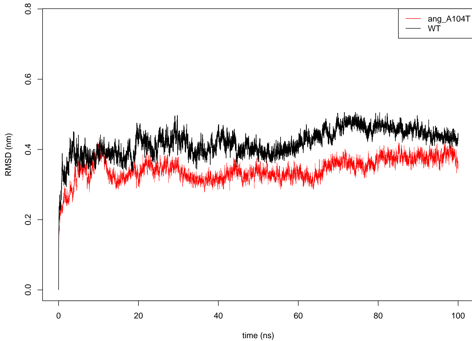
C alpha RMSD: ang_A104T vs WT
