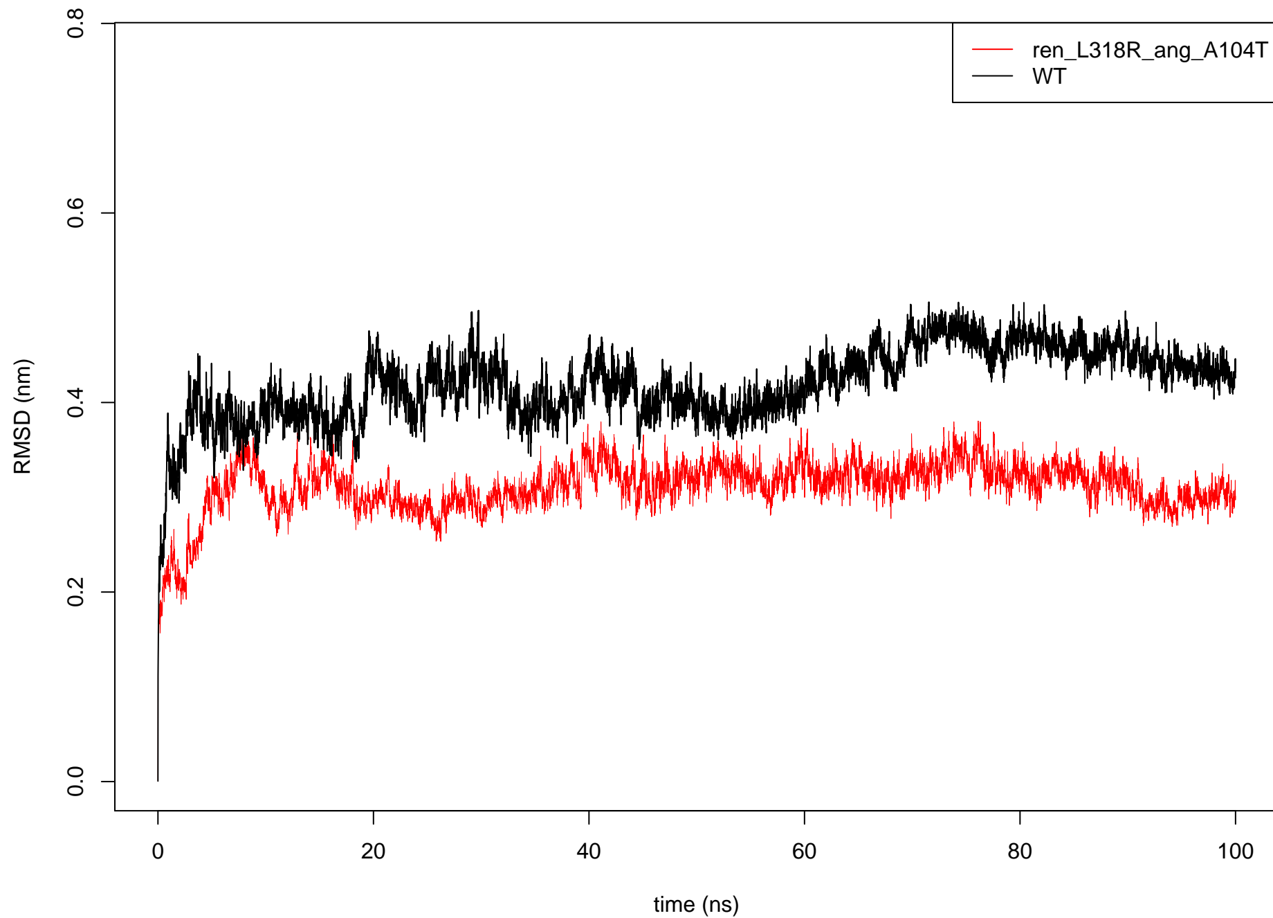
C alpha RMSD: ren_L318R_ang_A104T vs WT
