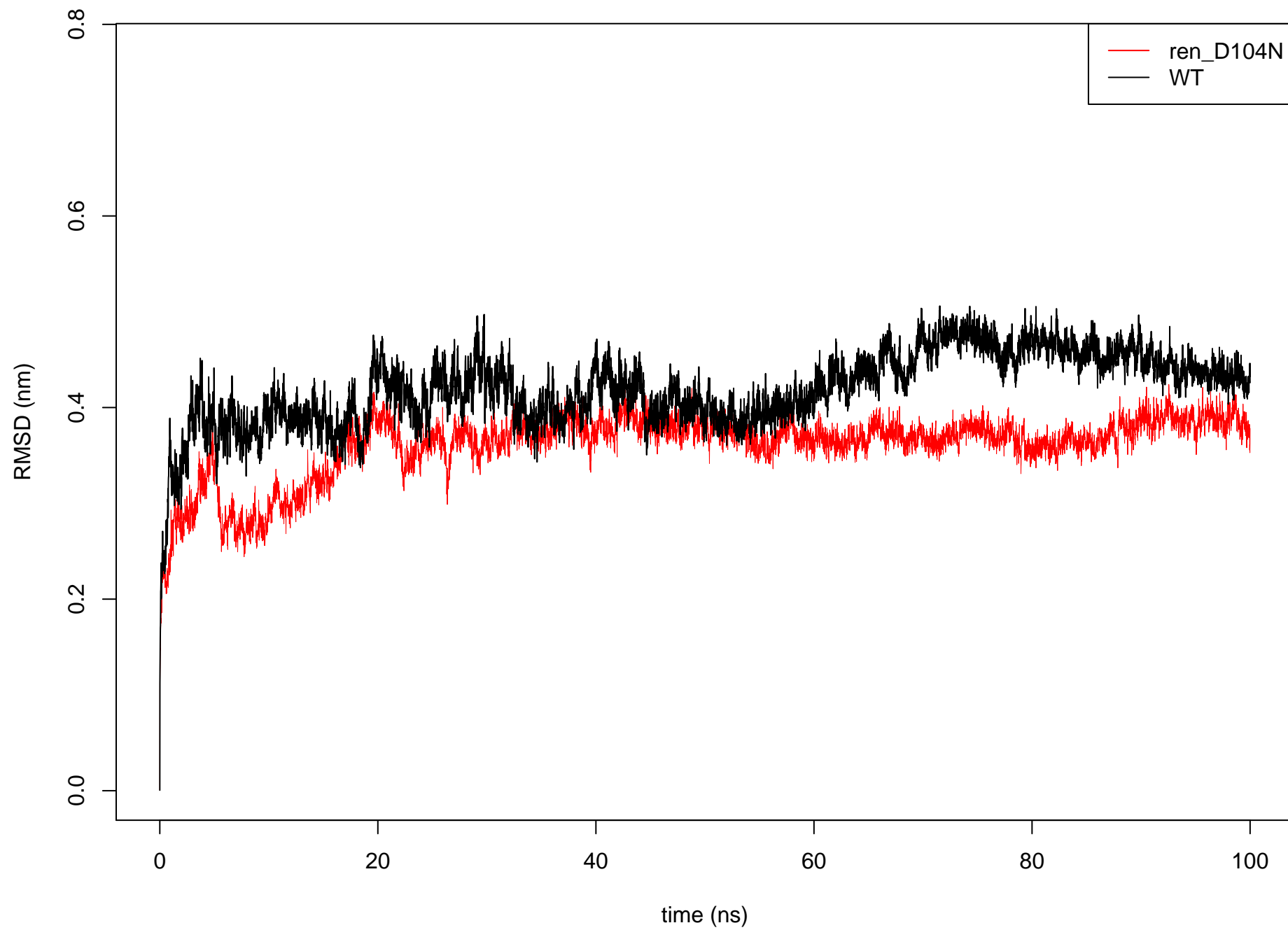
C alpha RMSD: ren_D104N vs WT
