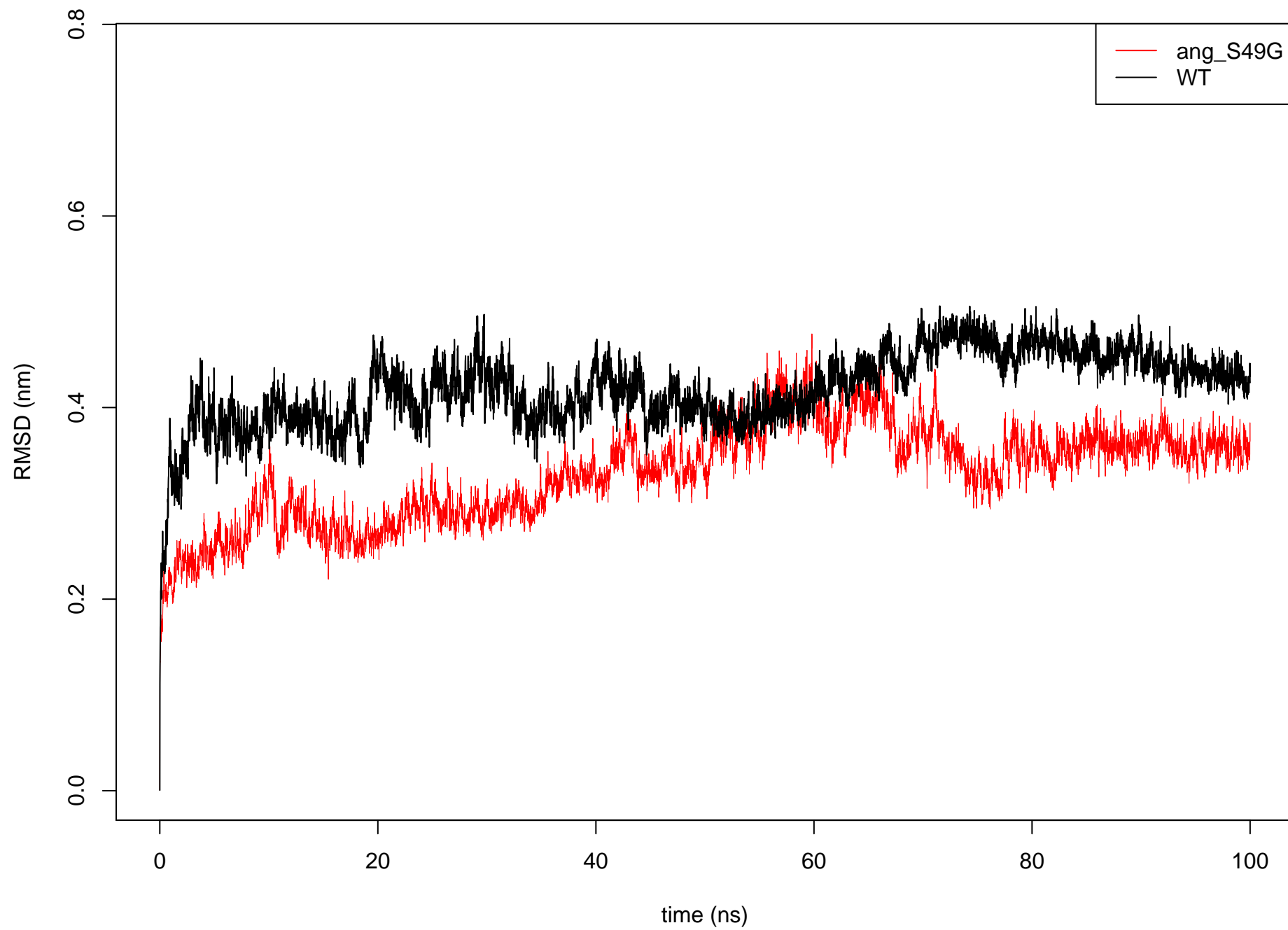
C alpha RMSD: ang_S49G vs WT
