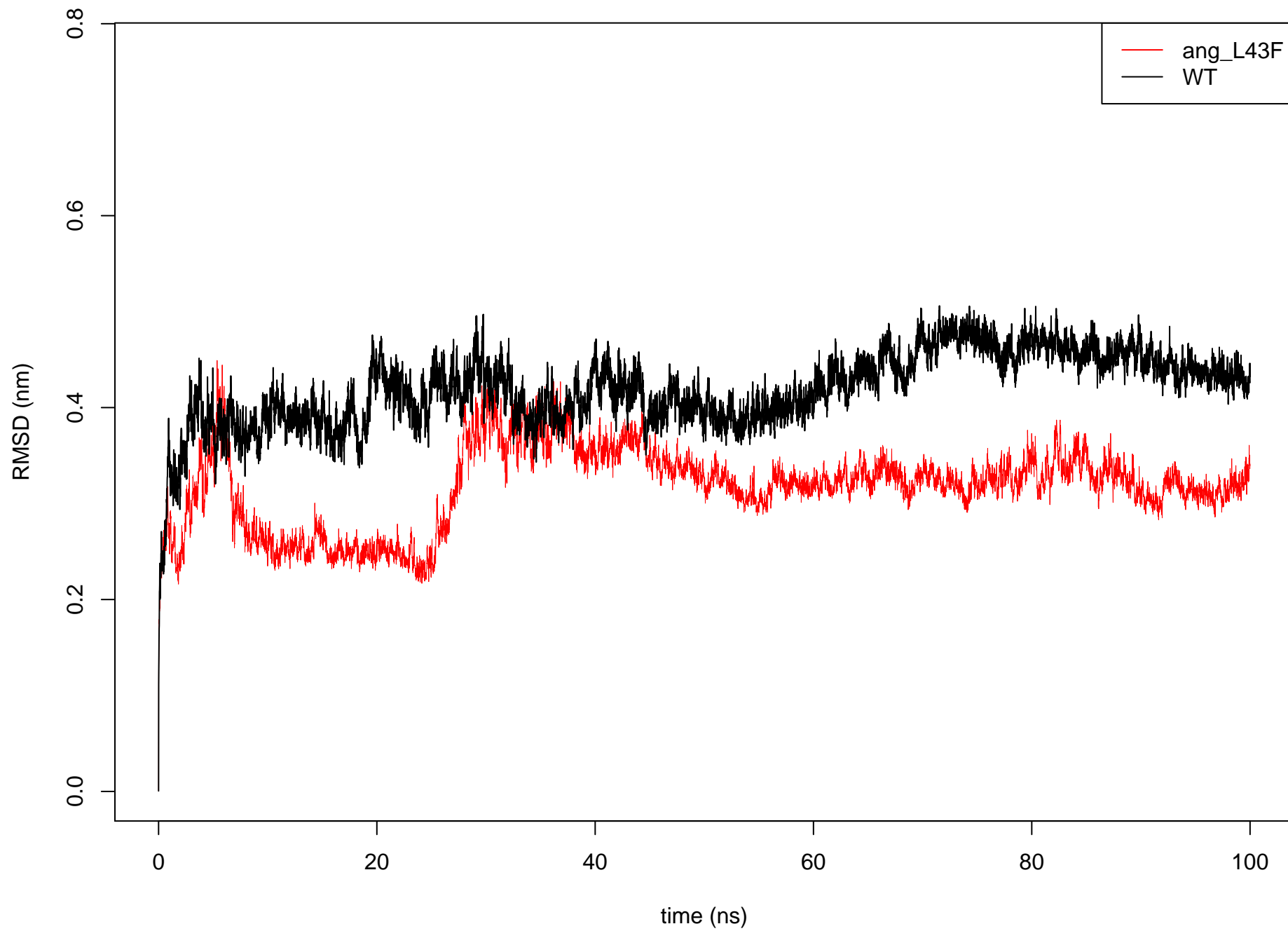
C alpha RMSD: ang_L43F vs WT
