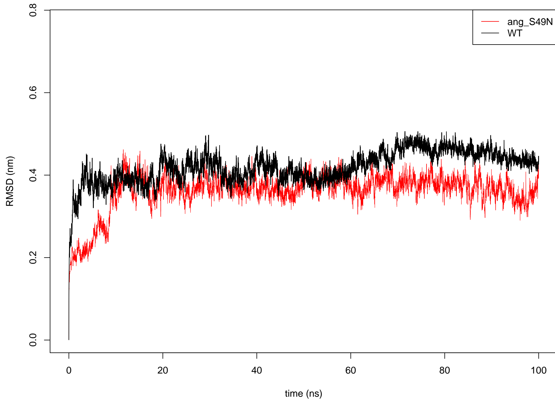
C alpha RMSD: ang_S49N vs WT
