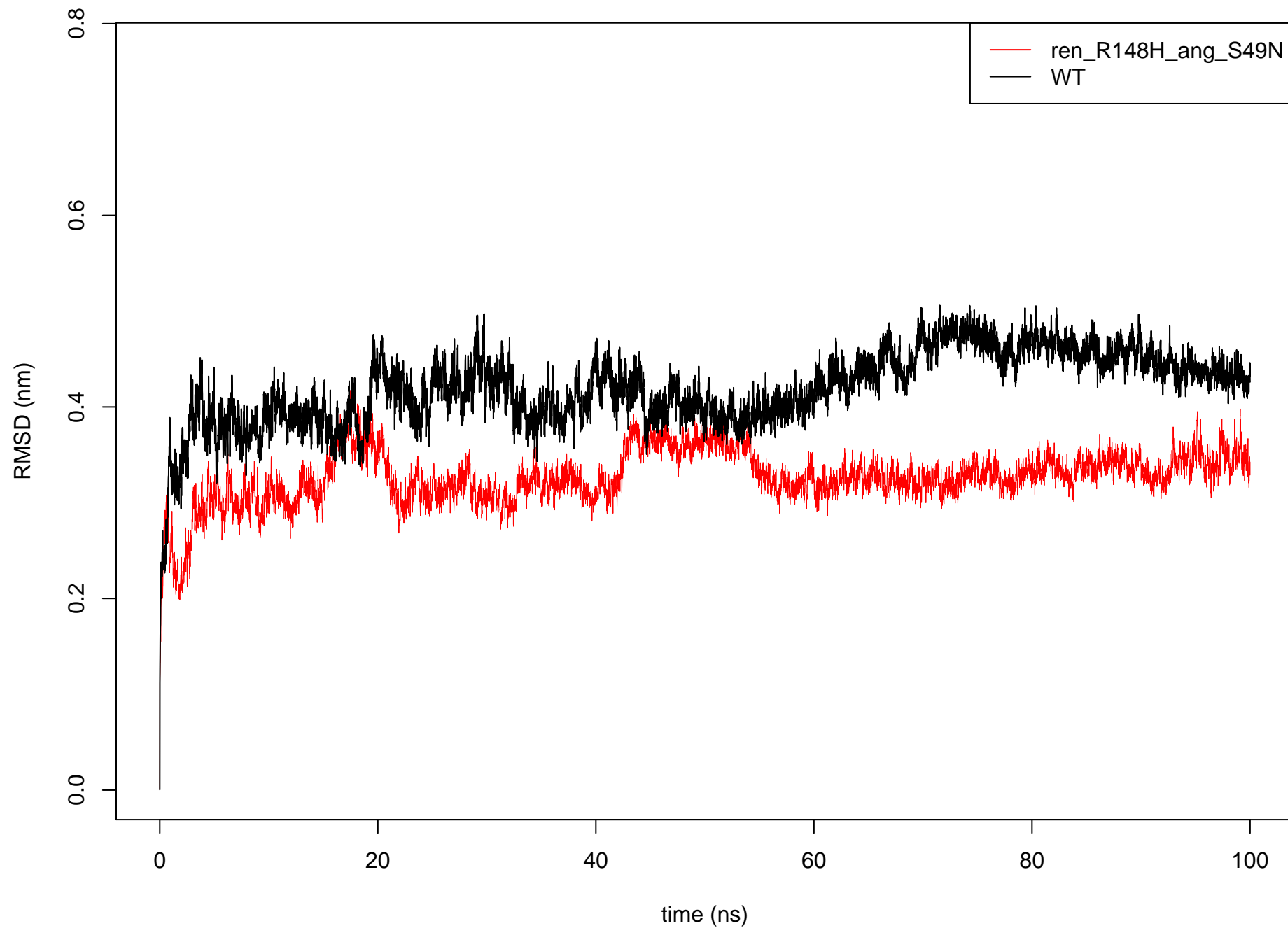
C alpha RMSD: ren_R148H_ang_S49N vs WT
