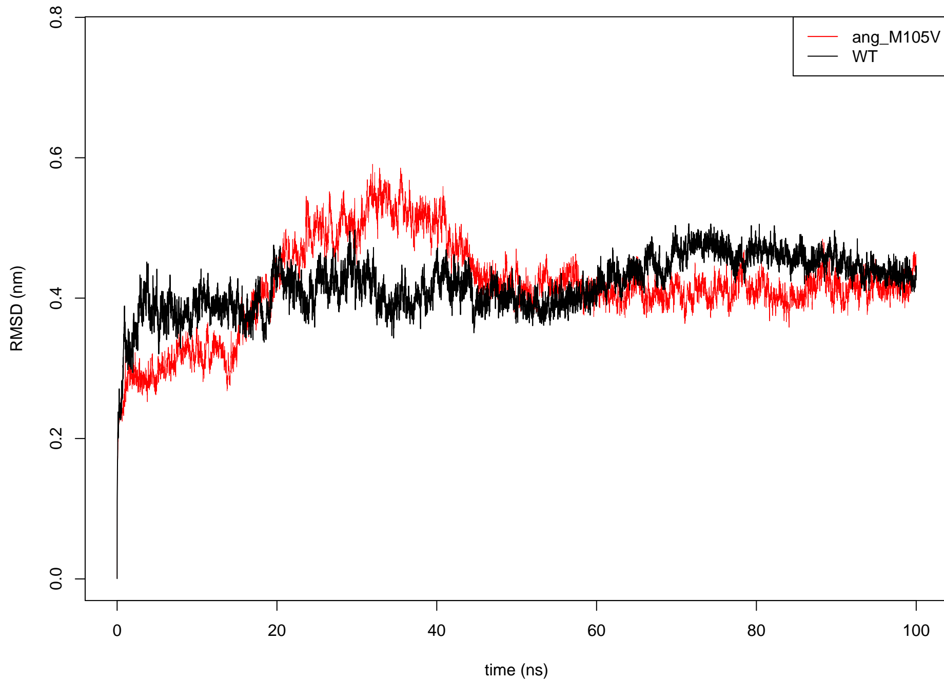
C alpha RMSD: ang_M105V vs WT
