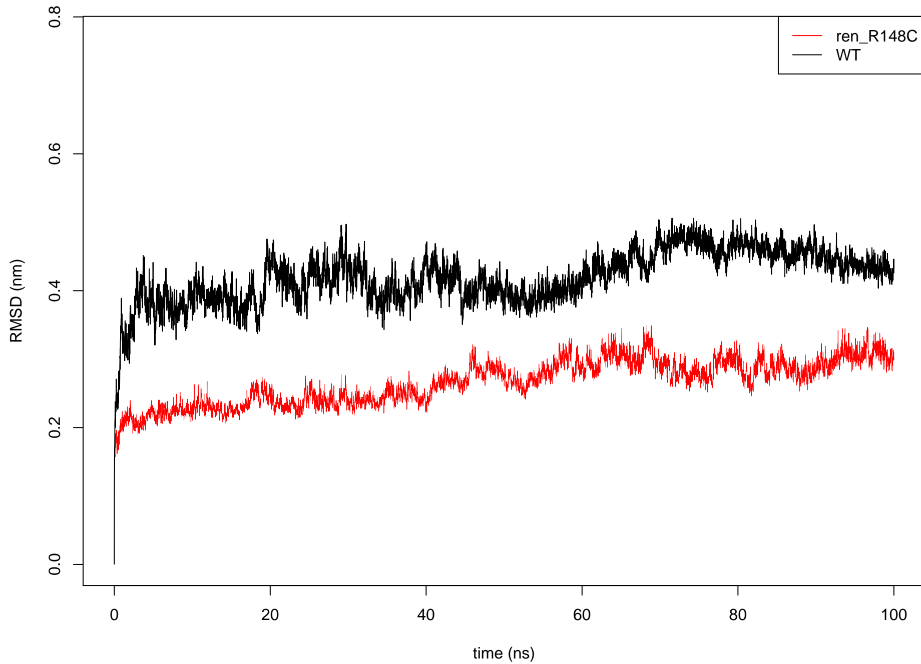
C alpha RMSD: ren_R148C vs WT
