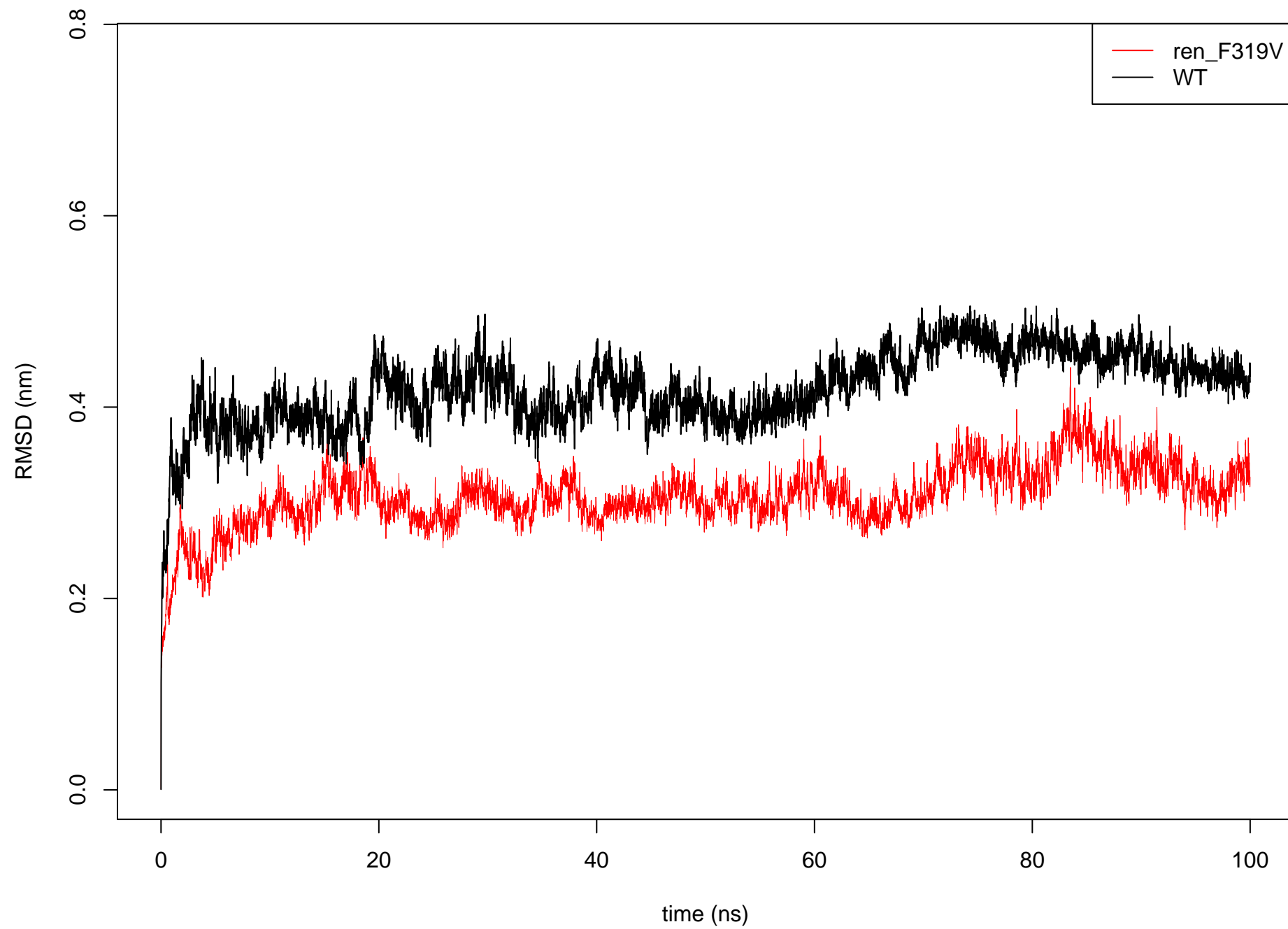
C alpha RMSD: ren_F319V vs WT
