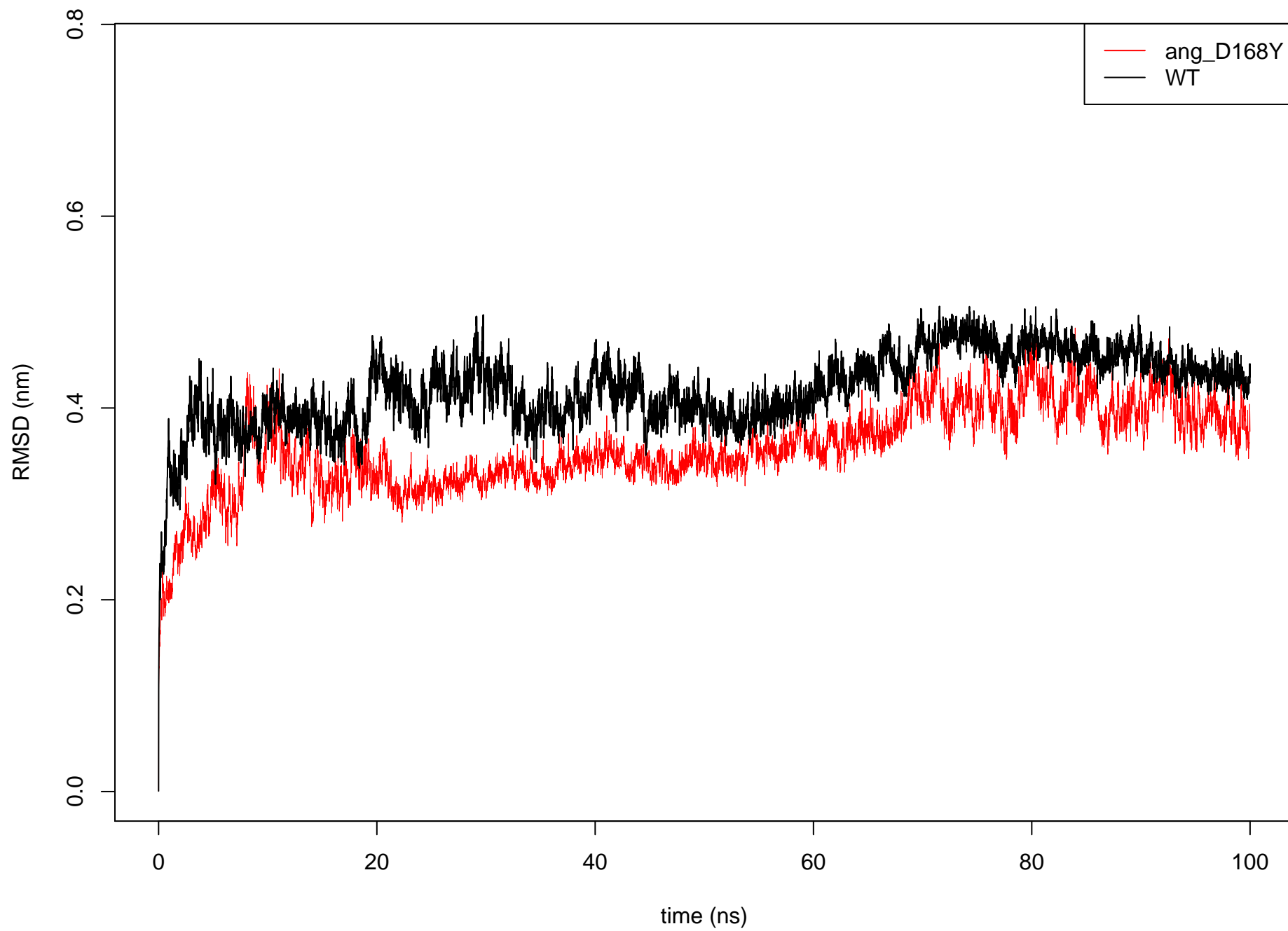
C alpha RMSD: ang_D168Y vs WT
