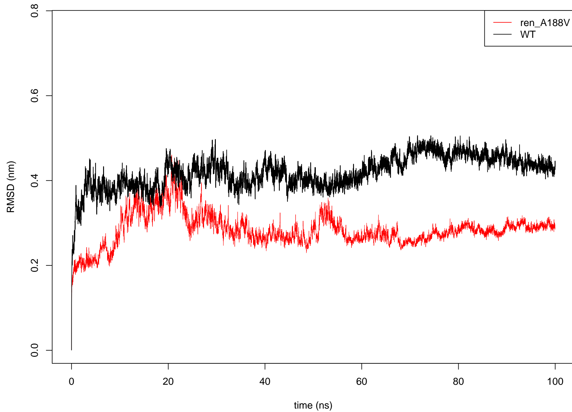
C alpha RMSD: ren_A188V vs WT
