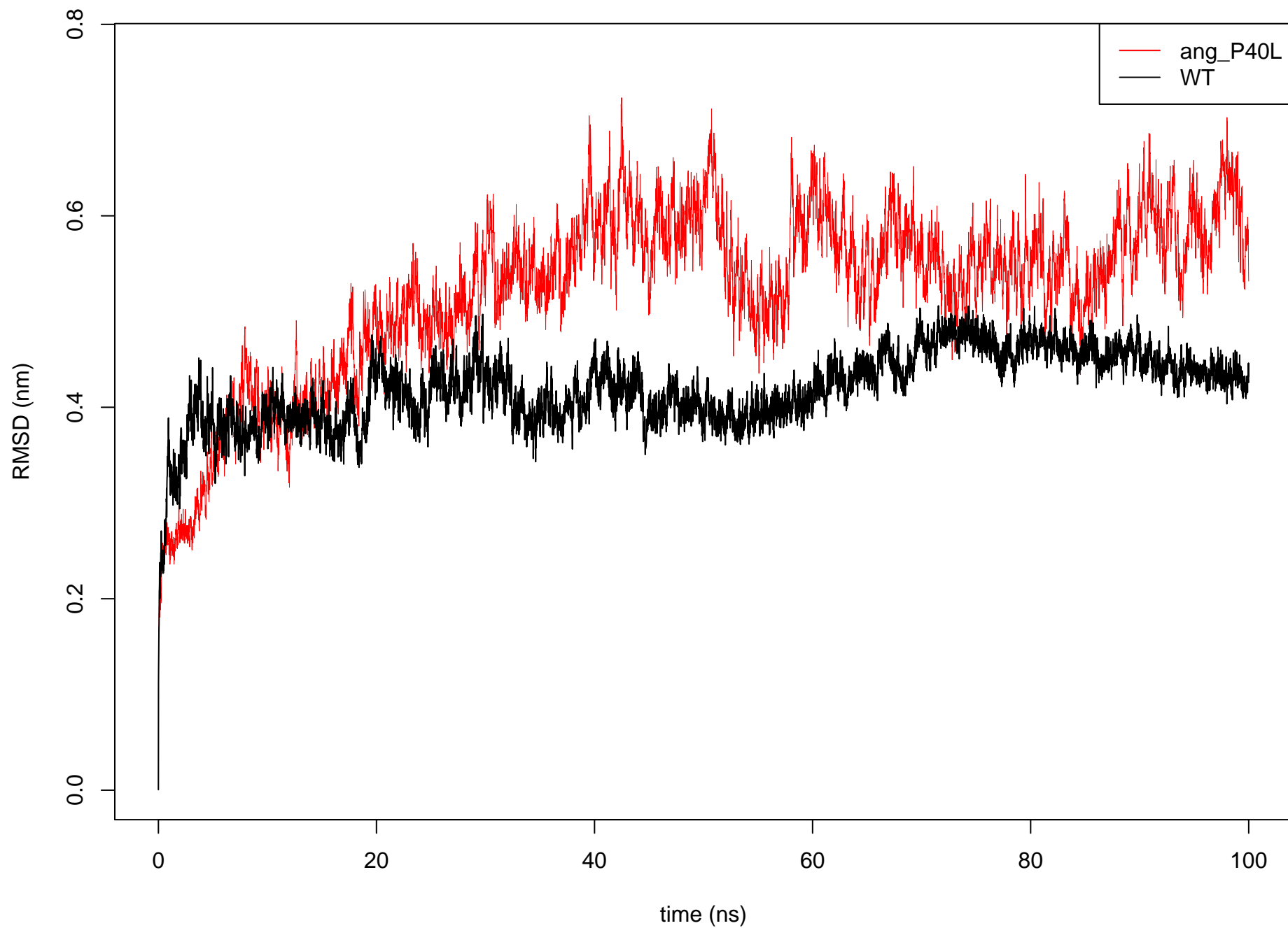
C alpha RMSD: ang_P40L vs WT
