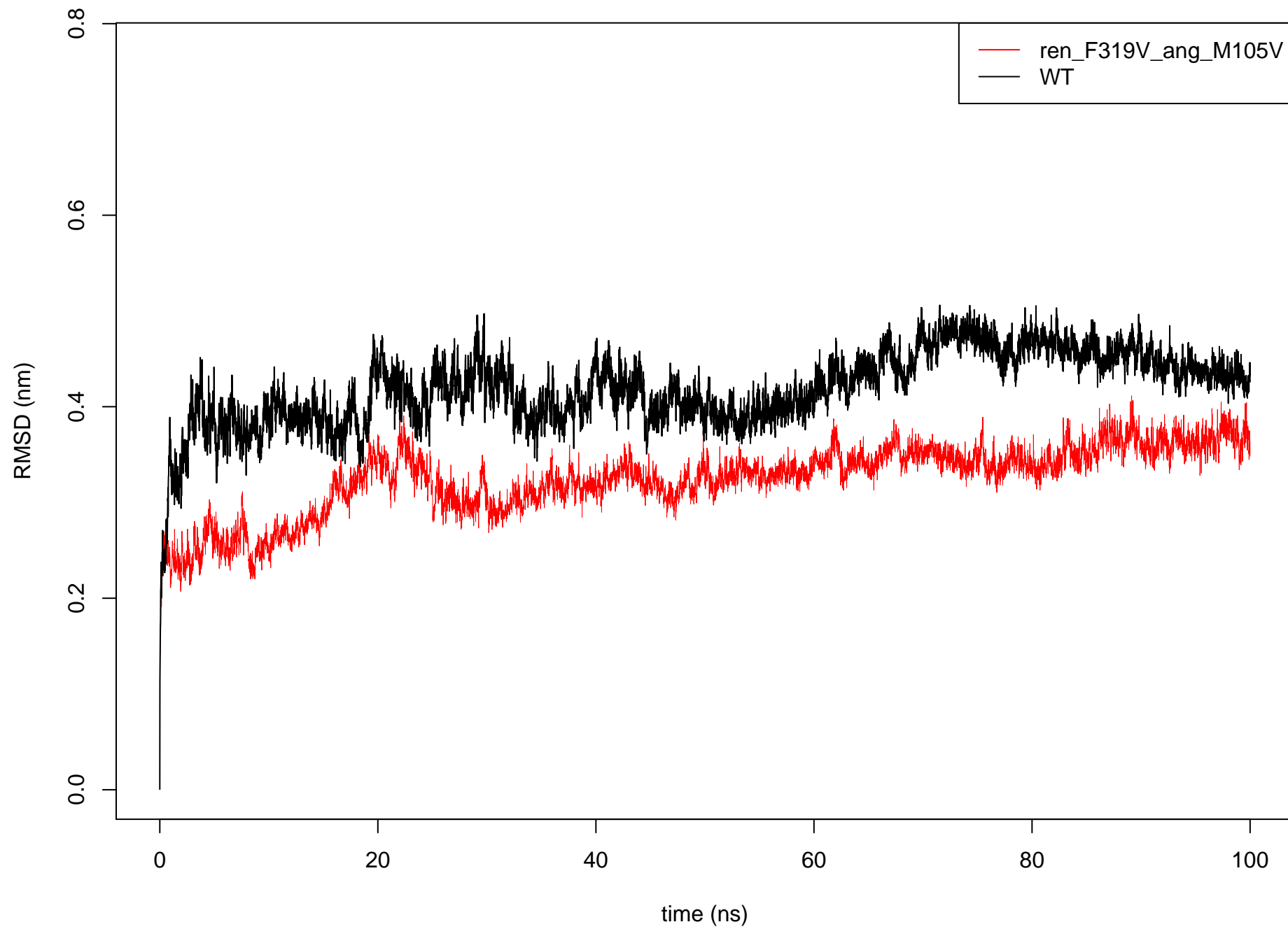
C alpha RMSD: ren_F319V_ang_M105V vs WT
