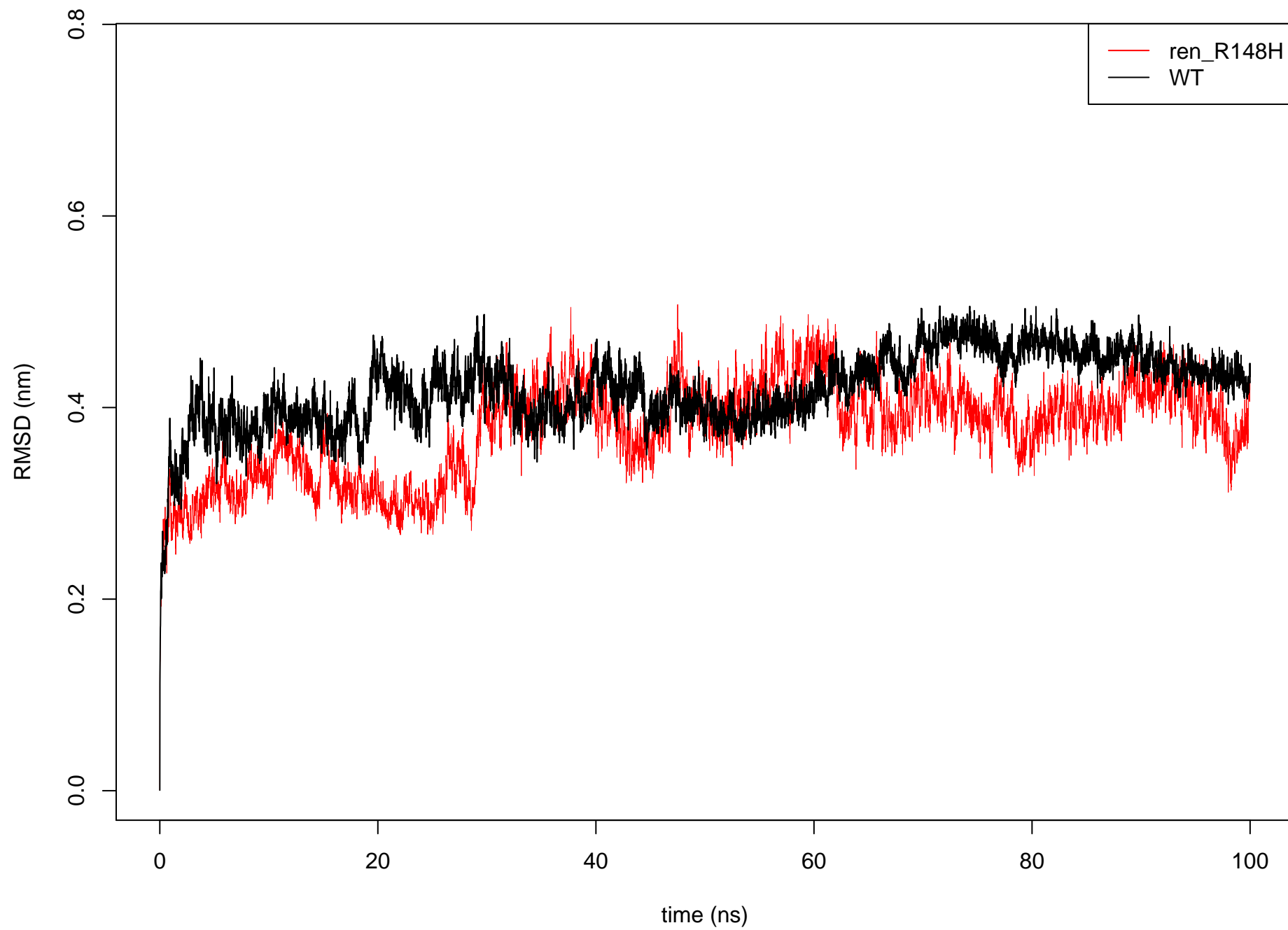
C alpha RMSD: ren_R148H vs WT
