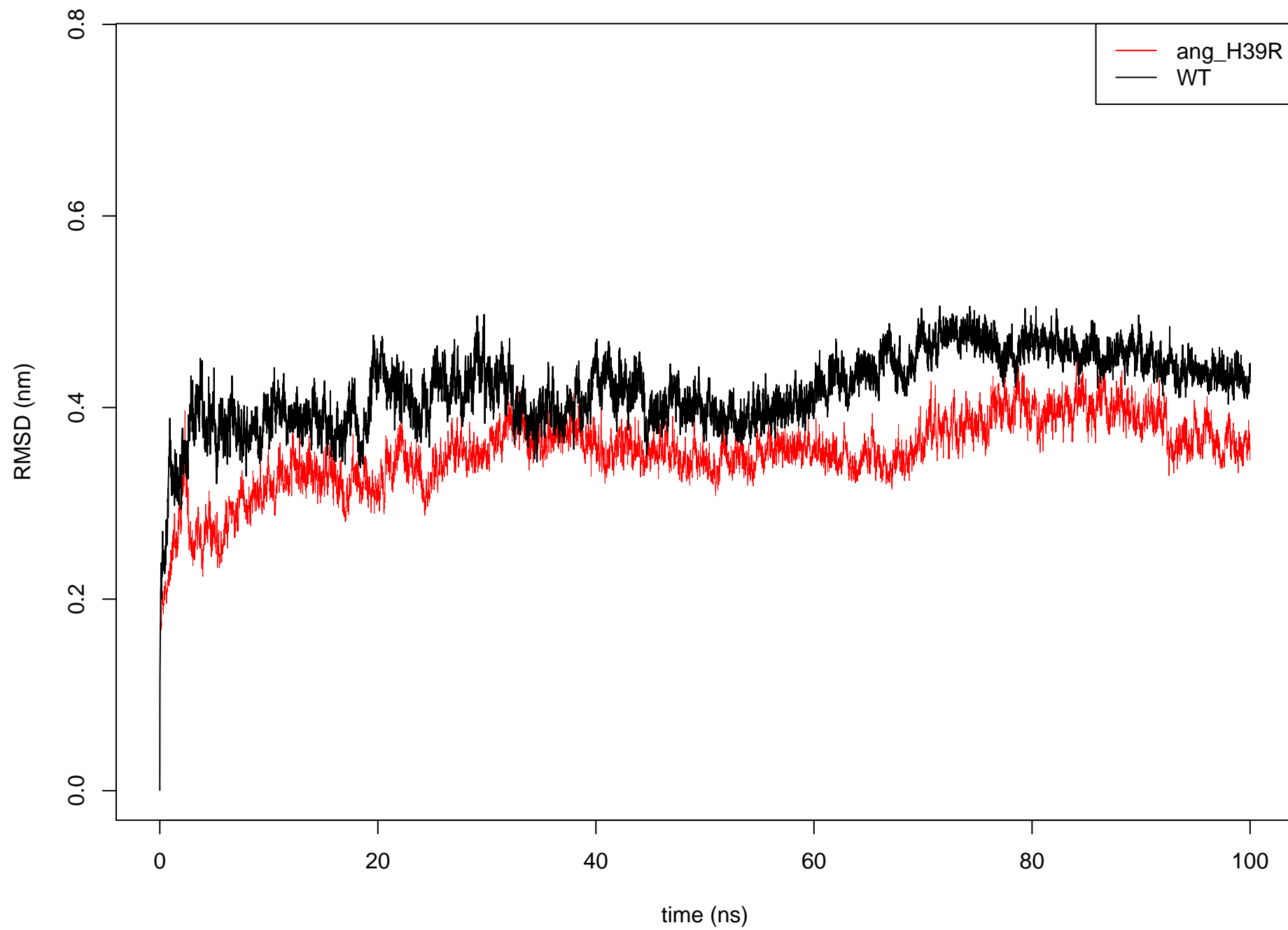
C alpha RMSD: ang_H39R vs WT
