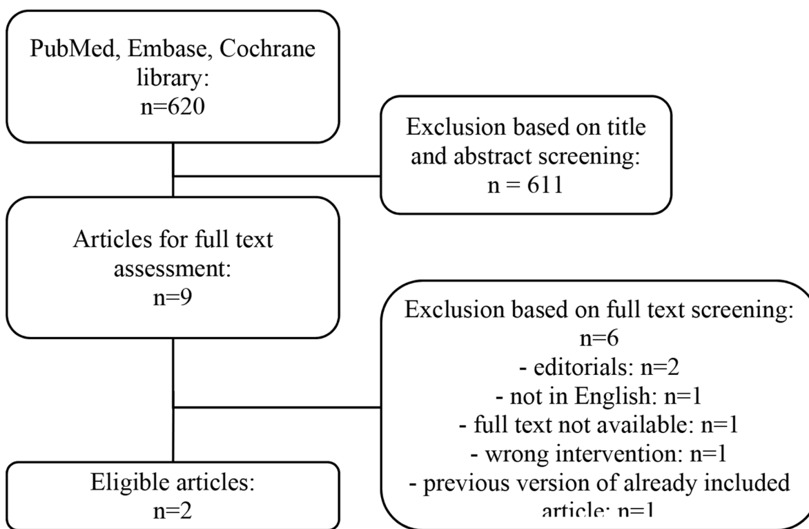
Supplementary Figure 1: Flow chart of search results from August 2013–November 2016.
