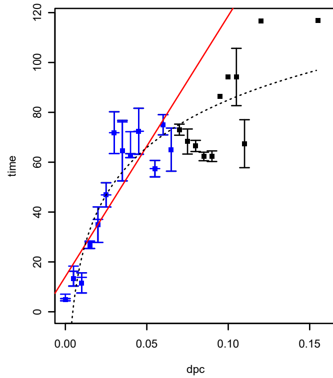
SPO3016 (COG0685) (*HTCC2255-Basal)
