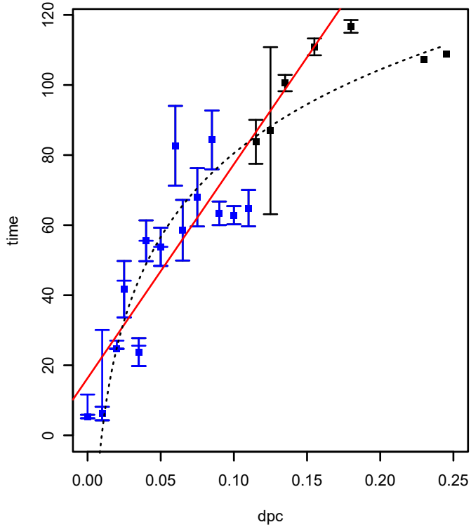
SPO0714 (COG2893) (*HTCC2255-Basal)
