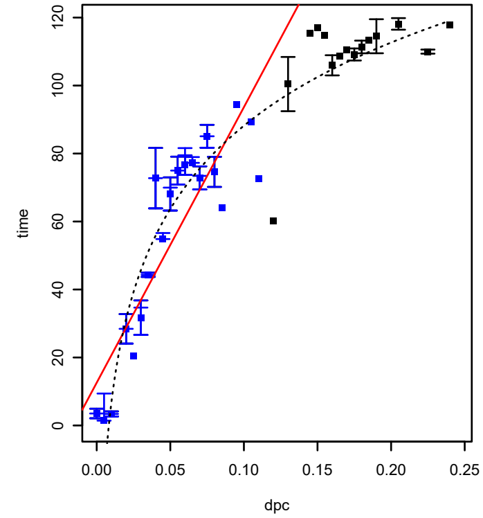
SPO3630 (COG0382) (*HTCC2255-Basal)
