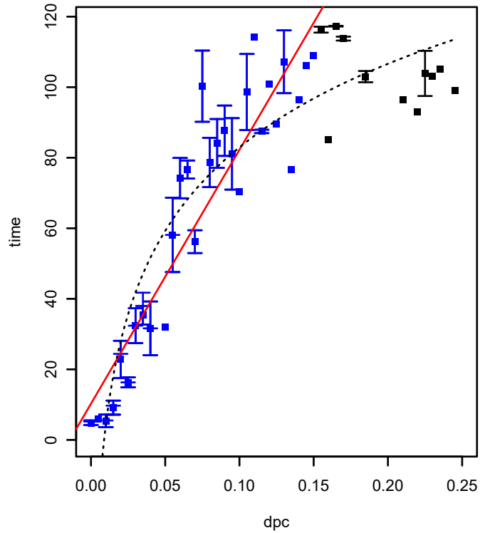
SPO2743 (COG1235) (*HTCC2255-Basal)
