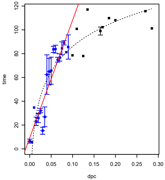
SPO3392 (COG0564) (*HTCC2255-Basal)
