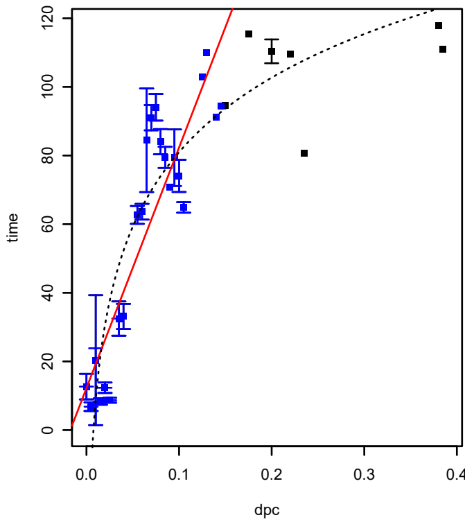
SPO2460 (COG2890) (*HTCC2255-Basal)
