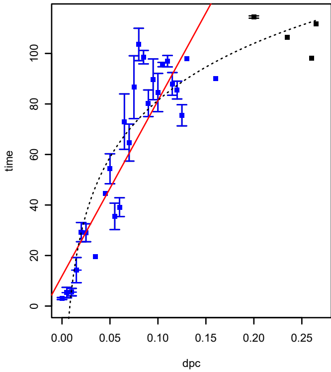
SPO3759 (COG1058) (*HTCC2255-Basal)
