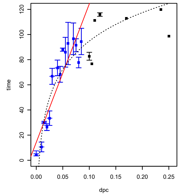
SPO3415 (COG2834) (*HTCC2255-Basal)
