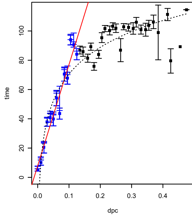
SPO1313 (NA) (*HTCC2255-Basal)
