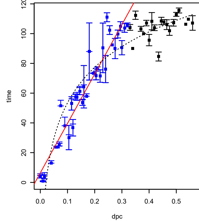
SPOA0008 (COG0319) (*HTCC2255-Basal)
