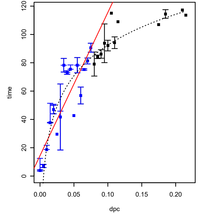
SPO3003 (COG0318) (*HTCC2255-Basal)
