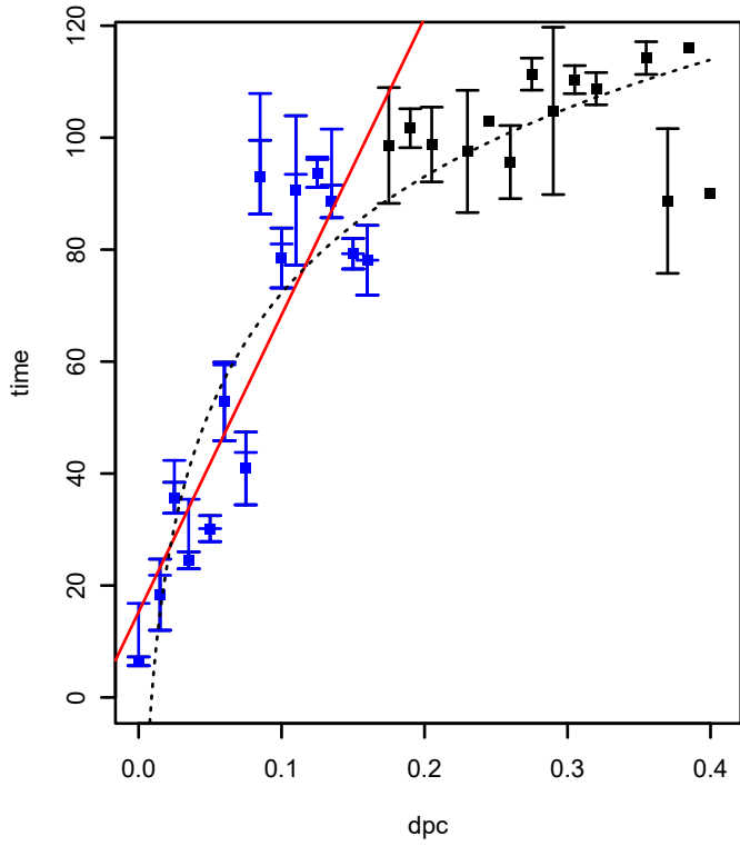
SPO0715 (COG1925) (*HTCC2255-Basal)
