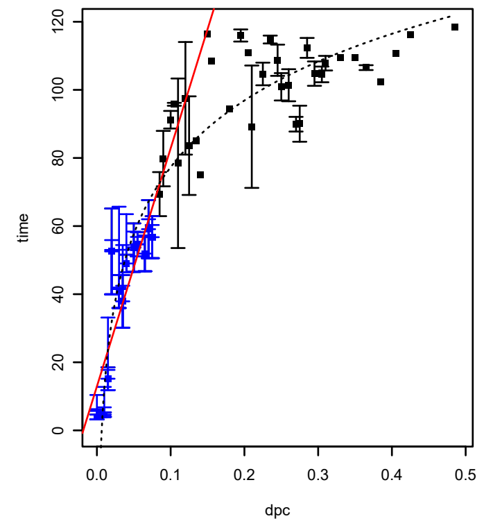
SPO2350 (COG0816) (*HTCC2255-Basal)
