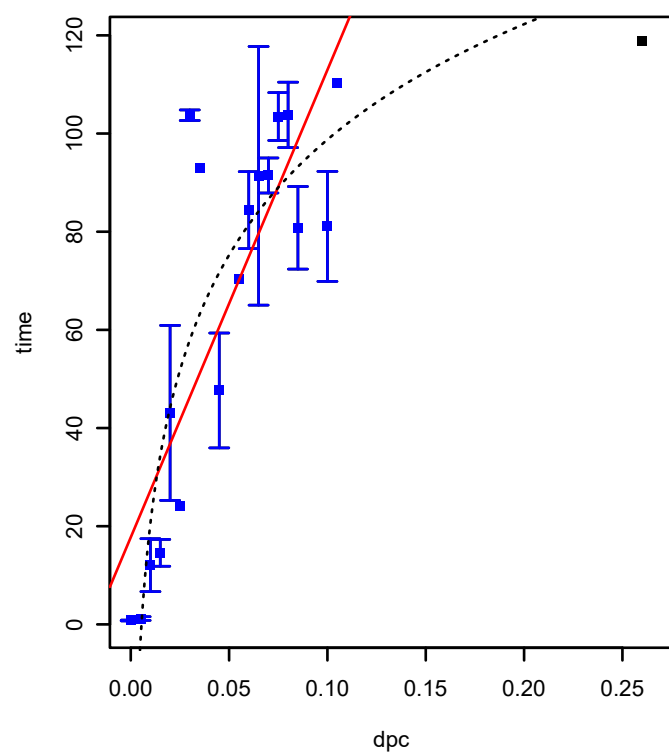
SPO3423 (COG3118) (*HTCC2255-Basal)
