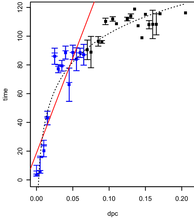
SPO3882 (COG1220) (*HTCC2255-Basal)
