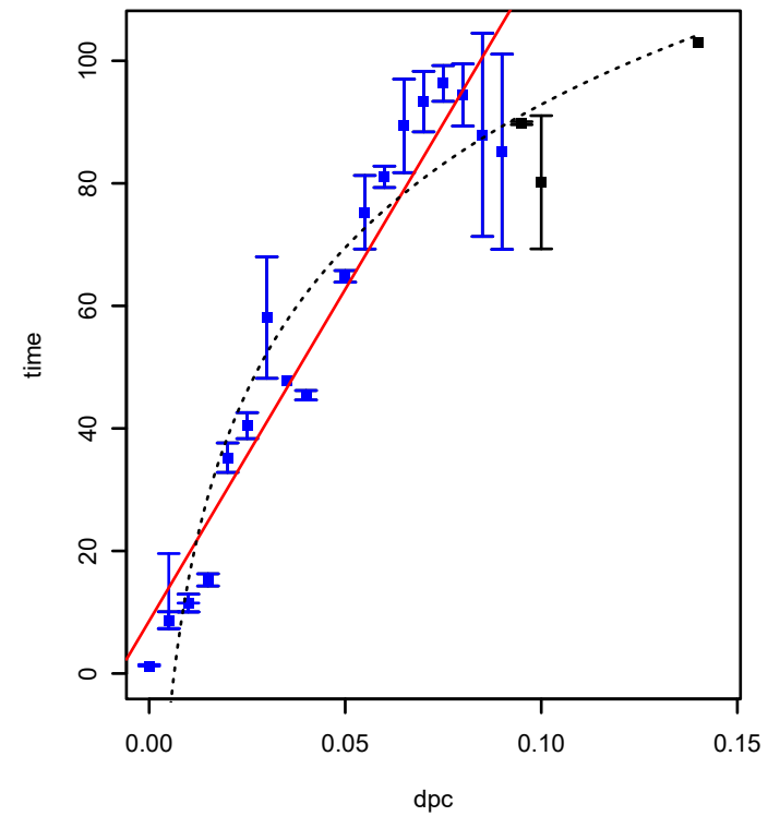
SPO1681 (COG1200) (*HTCC2255-Basal)
