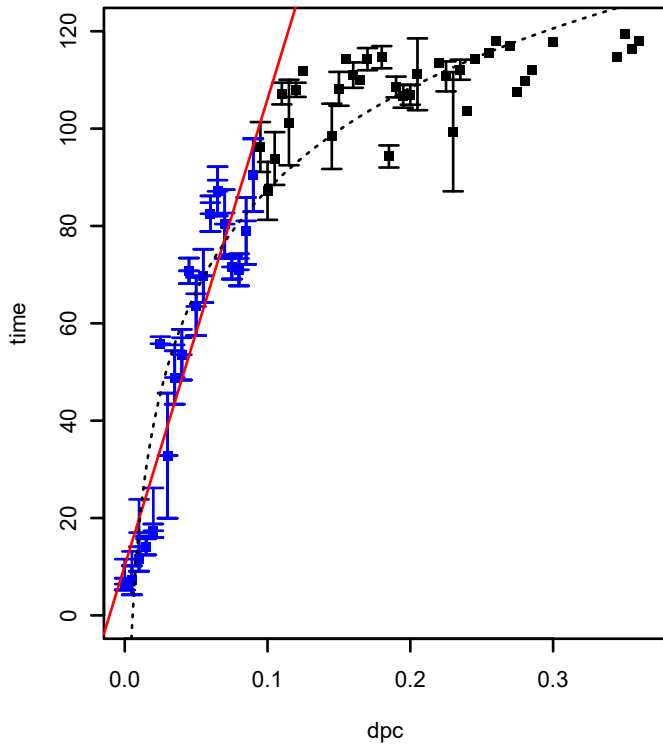
SPO2469 (COG3956) (*HTCC2255-Basal)
