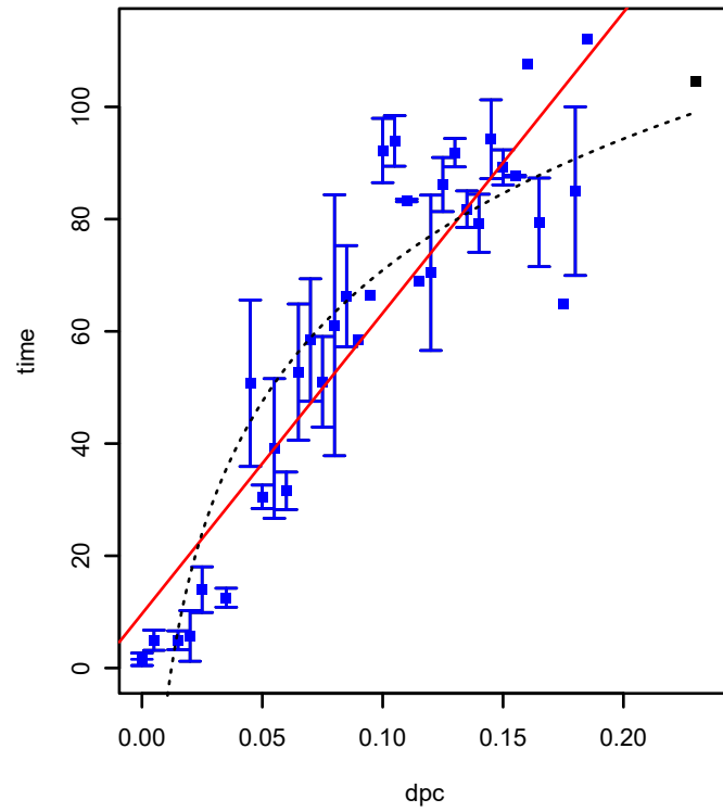
SPO3440 (COG4221) (*HTCC2255-Basal)
