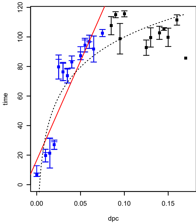
SPO3880 (COG5405) (*HTCC2255-Basal)
