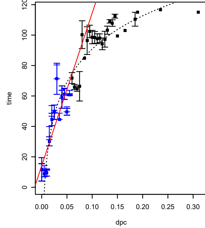
SPO3556 (COG0329) (*HTCC2255-Basal)
