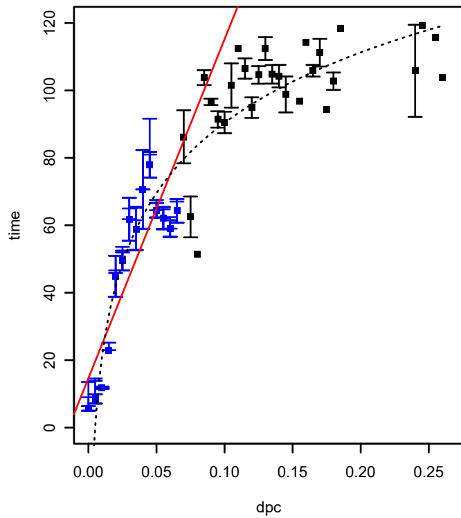
SPO2953 (COG1692) (*HTCC2255-Basal)
