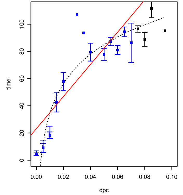
SPO3658 (COG1686) (*HTCC2255-Basal)
