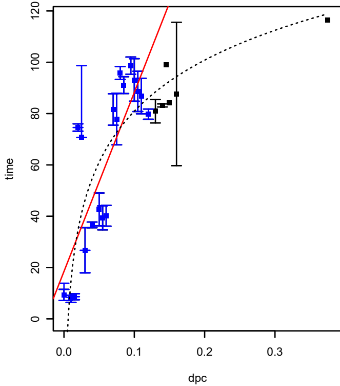
SPO1009 (COG2360) (*HTCC2255-Basal)
