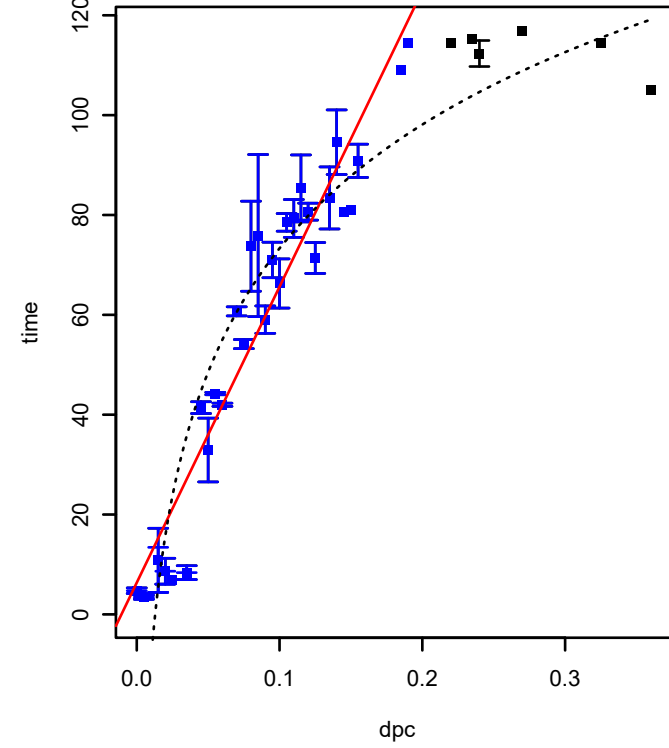
SPO1200 (COG0812) (*HTCC2255-Basal)
