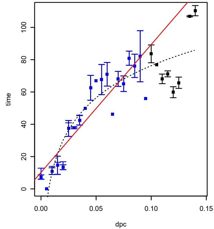
SPO3819 (COG1485) (*HTCC2255-Basal)
