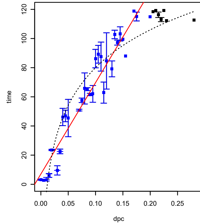
SPO3732 (COG3146) (*HTCC2255-Basal)
