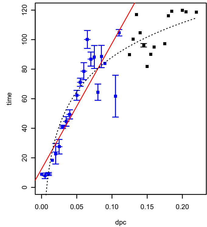
SPO2742 (COG0084) (*HTCC2255-Basal)
