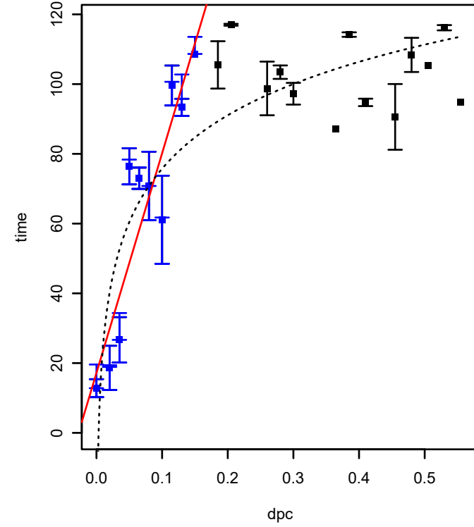
SPO0894 (COG5481) (*HTCC2255-Basal)
