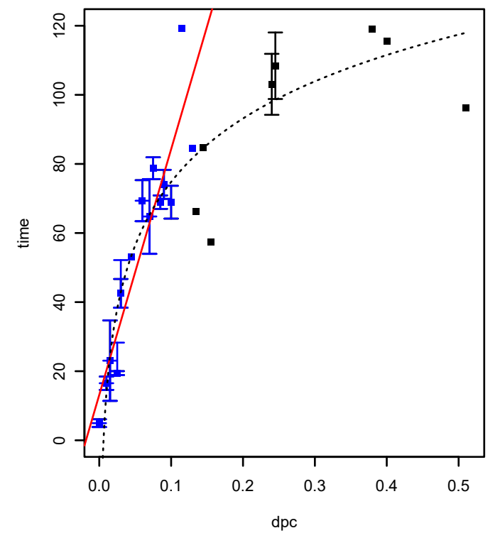
SPO1309 (COG4103) (*HTCC2255-Basal)
