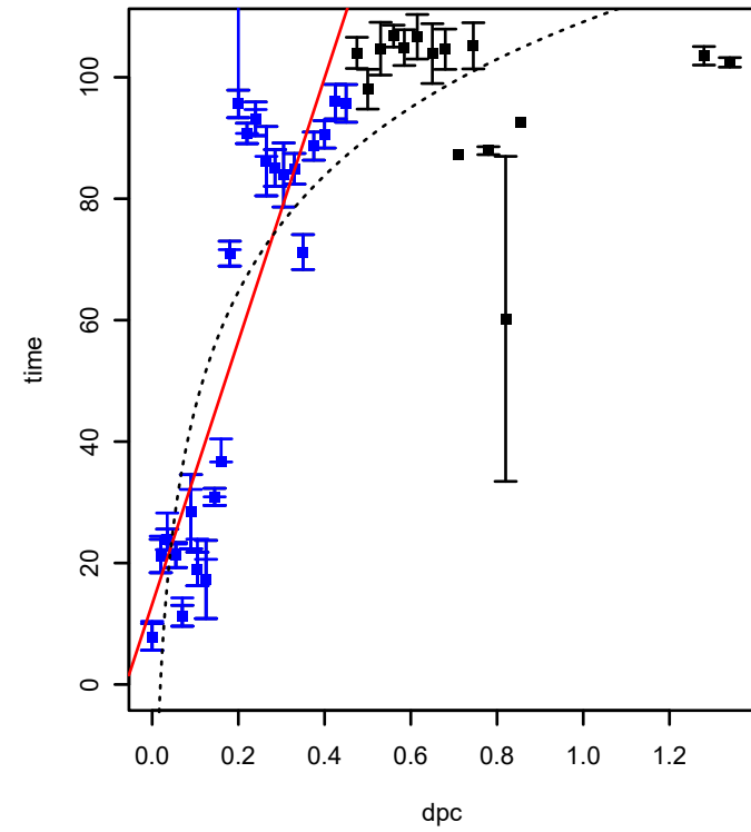
SPO0665 (COG2900) (*HTCC2255-Basal)
