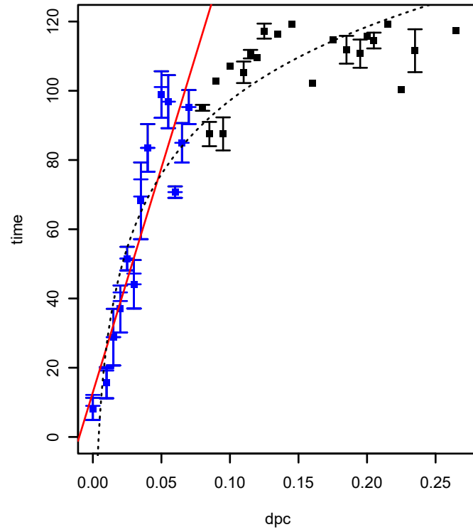
SPO3569 (COG0353) (*HTCC2255-Basal)
