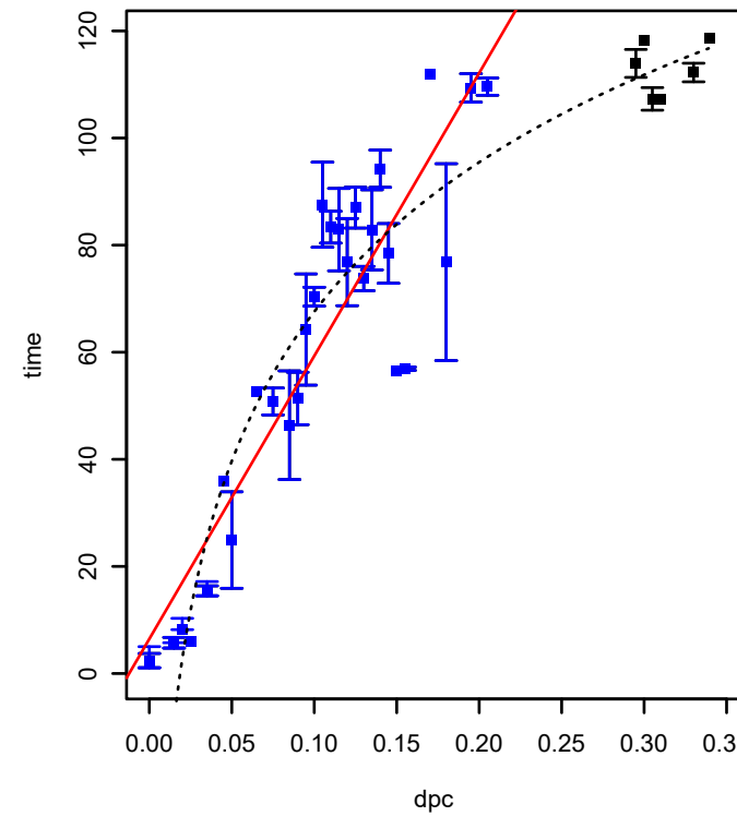
SPO1246 (COG0354) (*HTCC2255-Basal)
