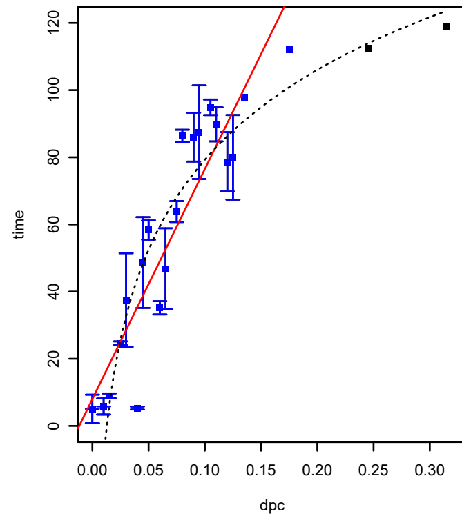
SPO1683 (COG0822) (*HTCC2255-Basal)
