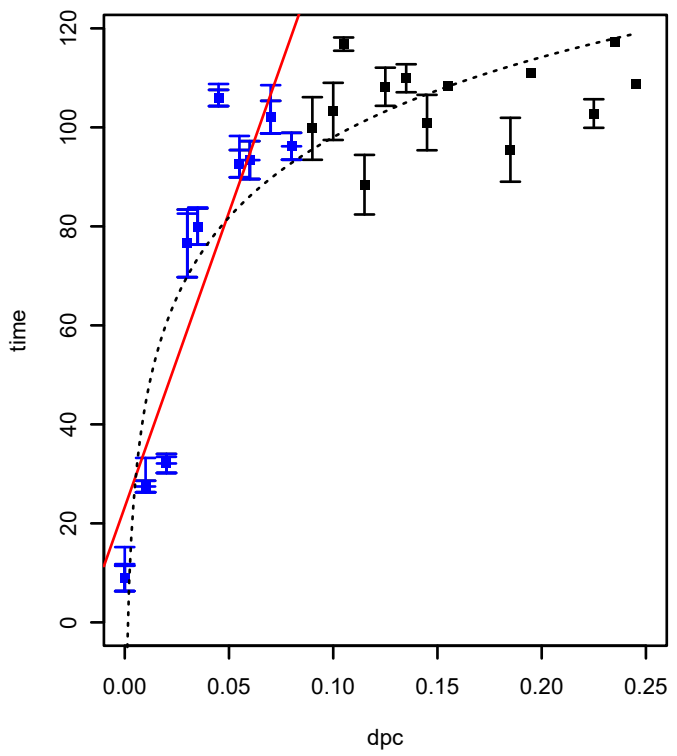
SPO2786 (COG0838) (*HTCC2255-Basal)
