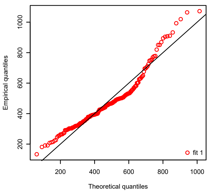
Q-Q plot
