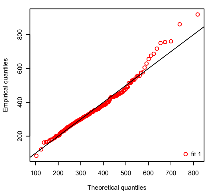
Q-Q plot
