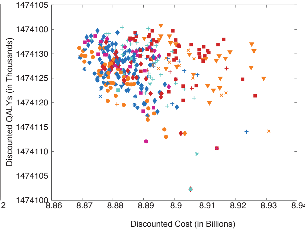
B Efficient frontiers varying cost and effectiveness of HIV interventions (N=100)
