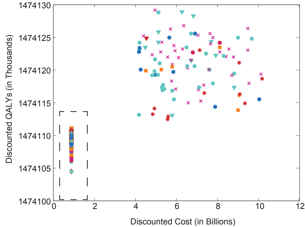
A Efficient frontiers varying cost and effectiveness of HIV interventions (N=100)
