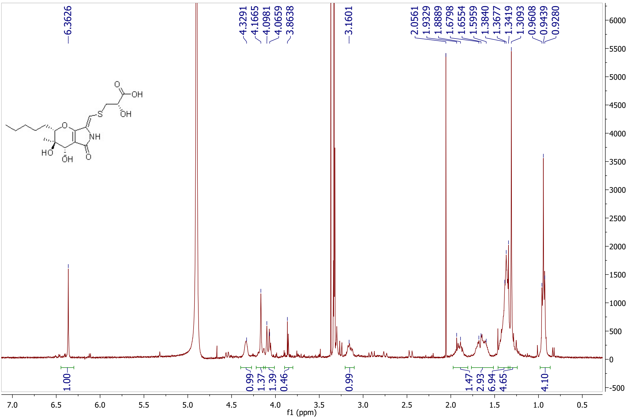
1 H NMR spectrum of compound 4 (400 MHz in methanol-d 4 )
