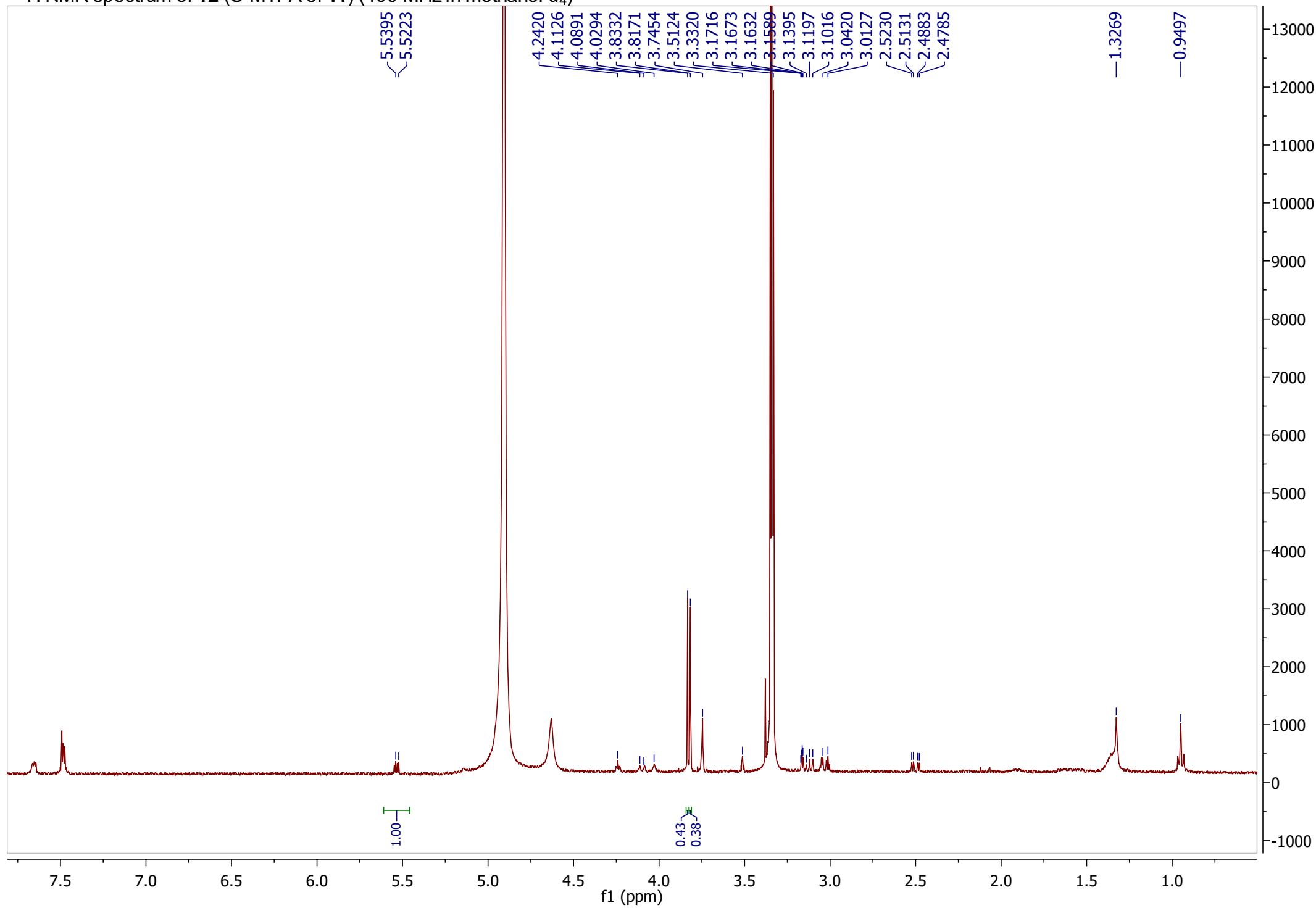
1 H NMR spectrum of 12 (S-MTPA of 11 ) (400 MHz in methanol- d 4 )
