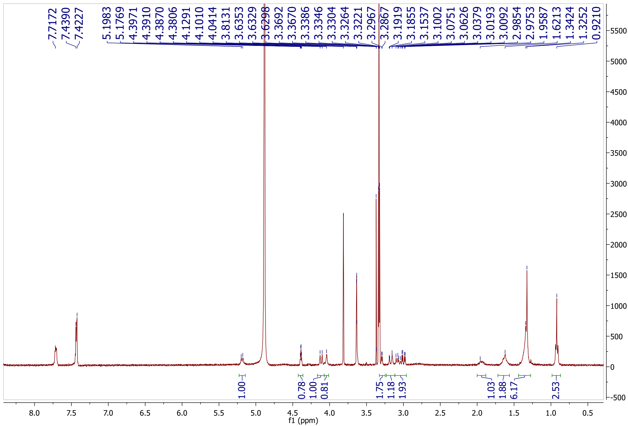
1 H NMR spectrum of compound 8 (S-MTPA of 1 ) (400 MHz in methanol-d 4 )
