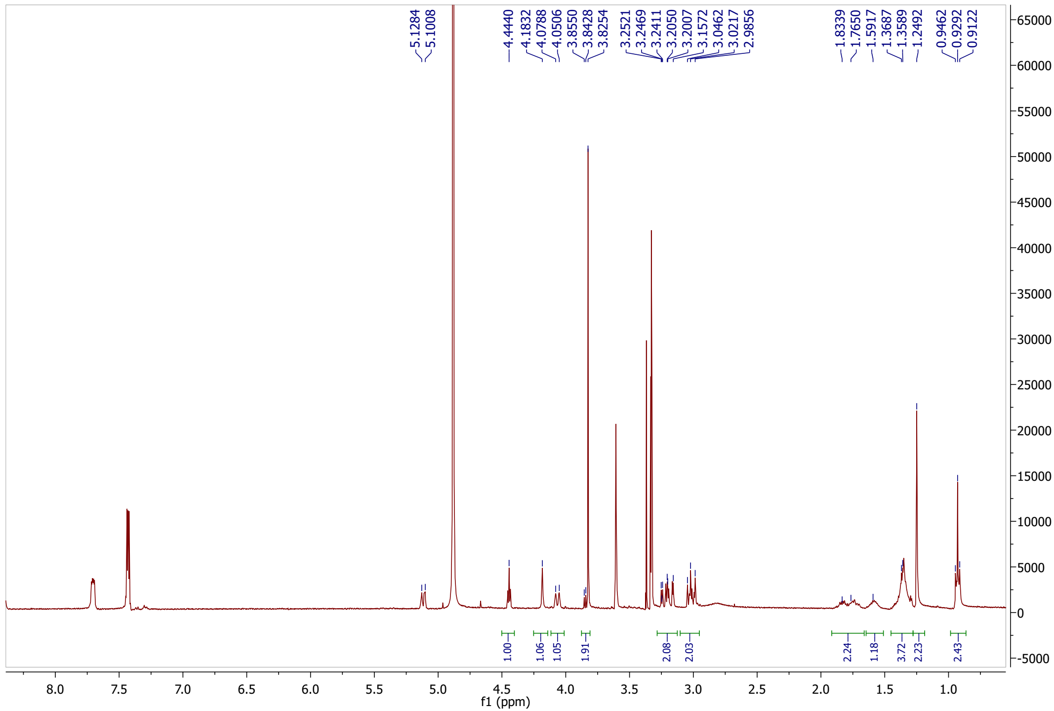
^1\text{H} NMR spectrum of compound 10 (S-MTPA of 2 ) (400 MHz in methanol- d_4 )
