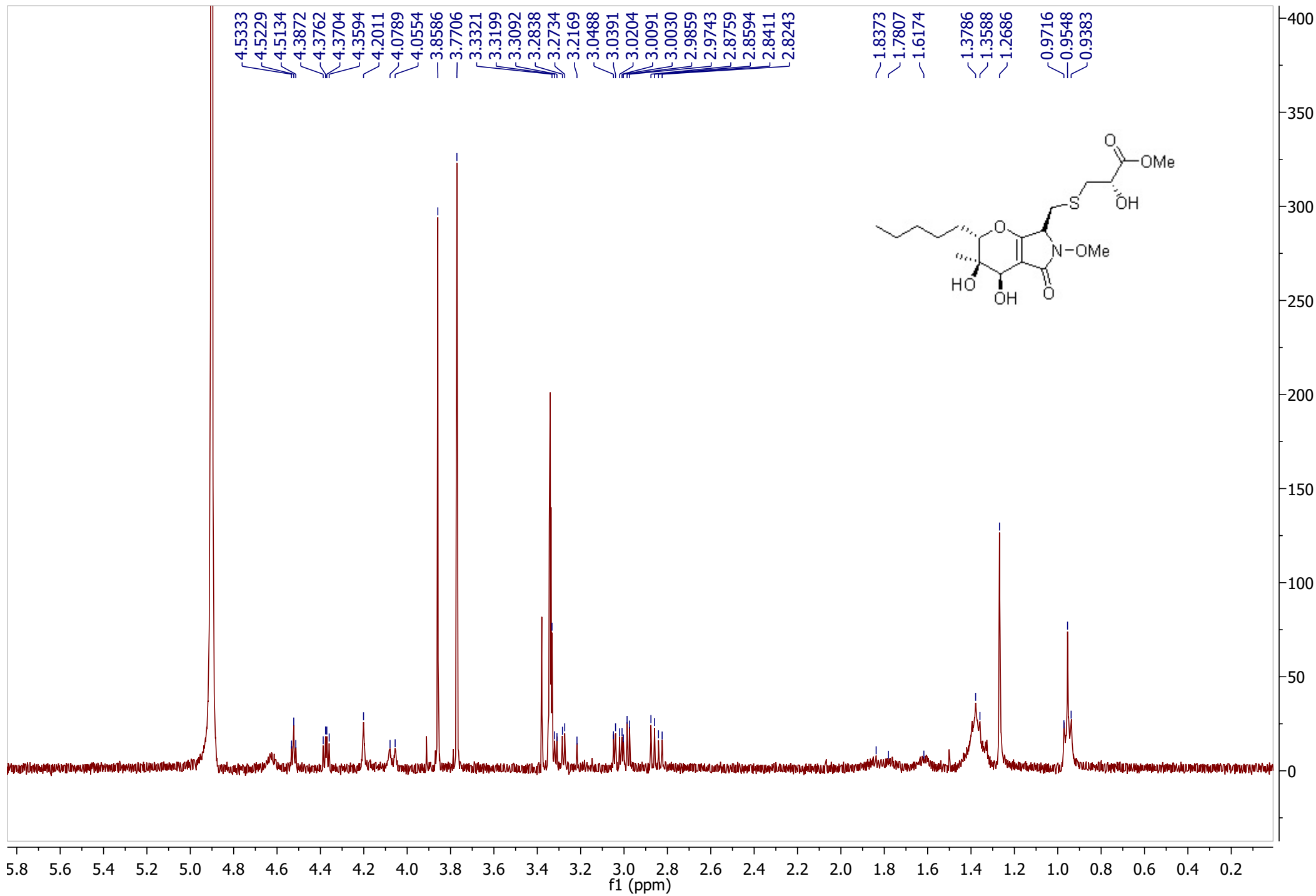
1 H NMR spectrum of compound 11 (400 MHz in methanol-d 4 )
