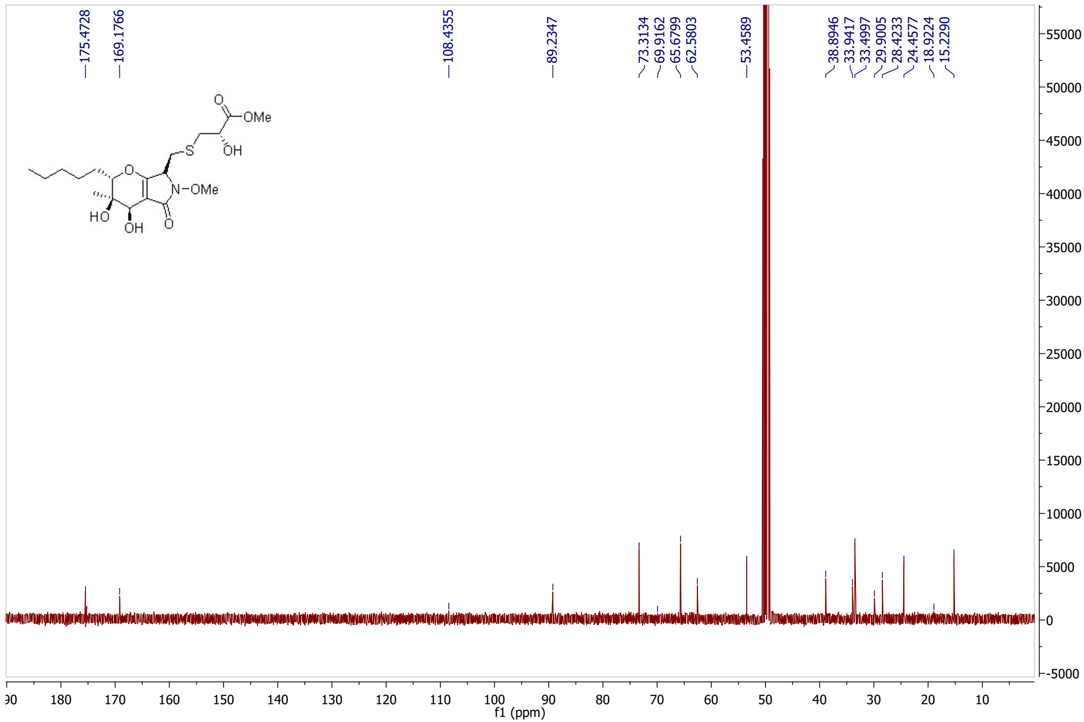
^{13}\text{C} NMR spectrum of compound 11
