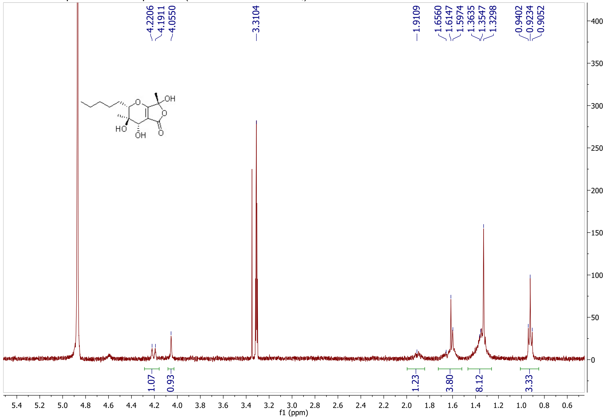
1 H NMR spectrum of compound 5 (400 MHz in methanol- d 4 )
