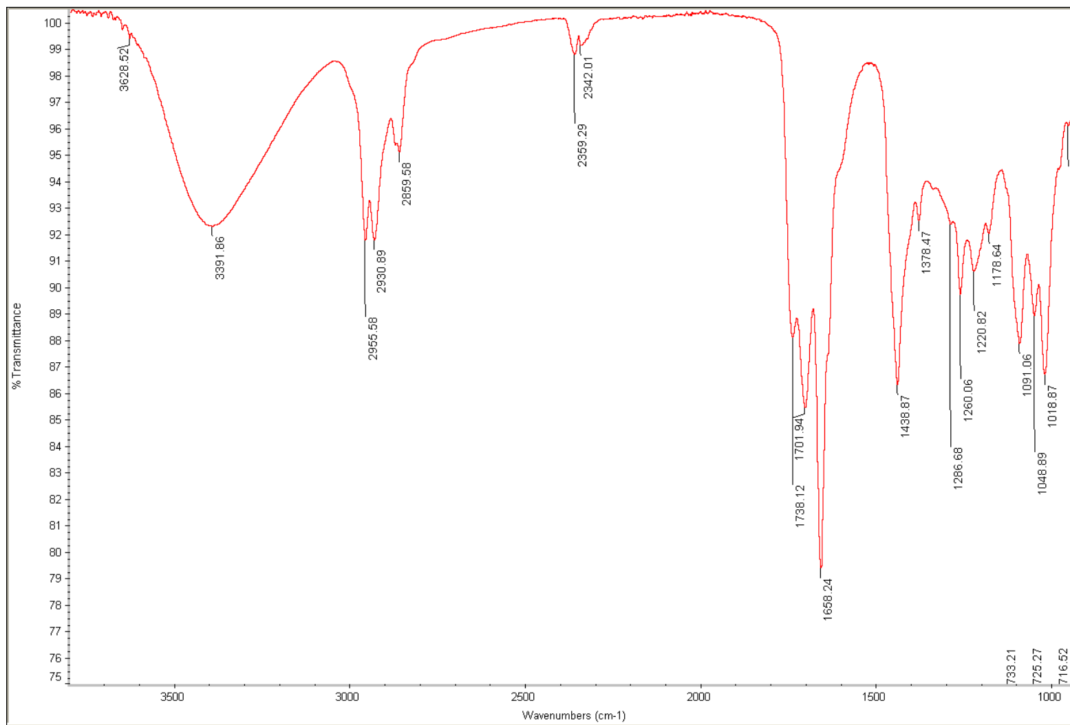
IR spectrum of compound 11
