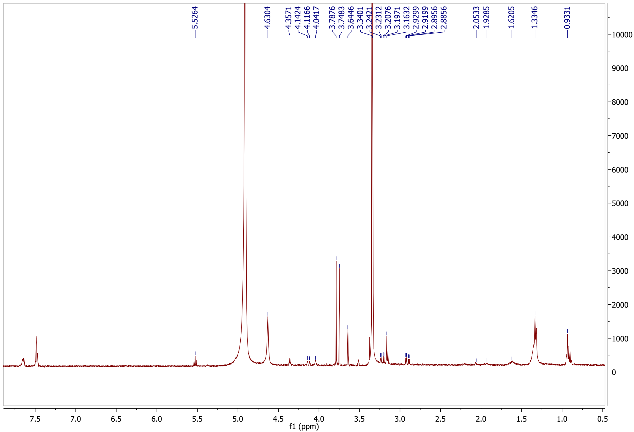
1 H NMR spectrum of 13 (R-MTPA of 11 ) (400 MHz in methanol- d 4 )
