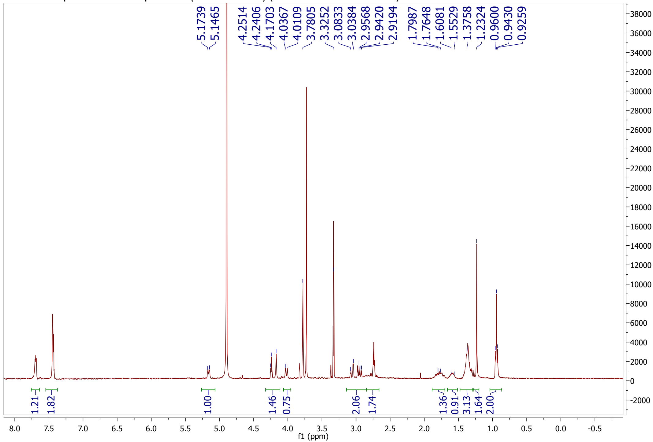
^1\text{H} NMR spectrum of compound 9 ( R -MTPA of 1 ) (400 MHz in methanol- d_4 )
