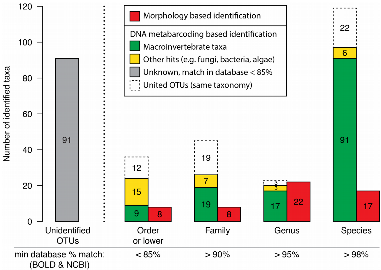
Figure S9: Comparison of macroinvertebrate taxa identified by DNA metabarcoding and morphological determination on different taxonomic levels. Below the bars the minimum required % match of the reference sequences required for sorting sequences into the respective category. OTUs with the same taxonomic hits in the reference database were merged into one single hit.
