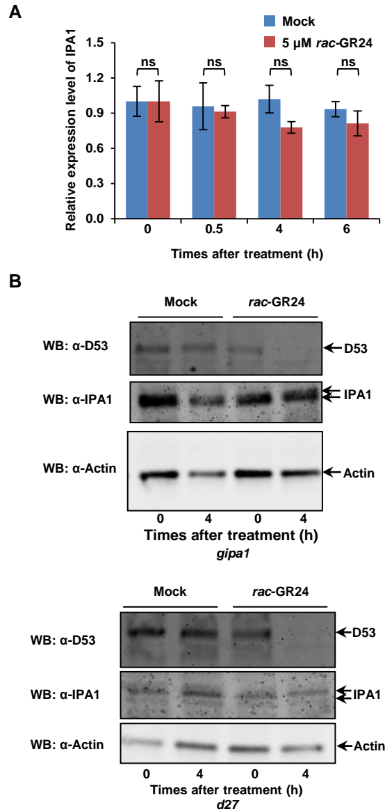
Figure S3 Expression and protein levels of IPA1 after rac -GR24 treatment. (A) Expression levels of IPA1 after rac -GR24 treatment. Rice Actin1 was used as a reference. Values are means \pm SE ( n = 3 ). Statistical difference was determined by Student's t test ( n = 3 ). ns, no significant difference. (B) Protein levels of IPA1 and D53 after rac -GR24 treatment in ipa1-1D genomic sequence transgenic line ( gipa1 ) and d27 mutant. Actin was used as the loading control.
