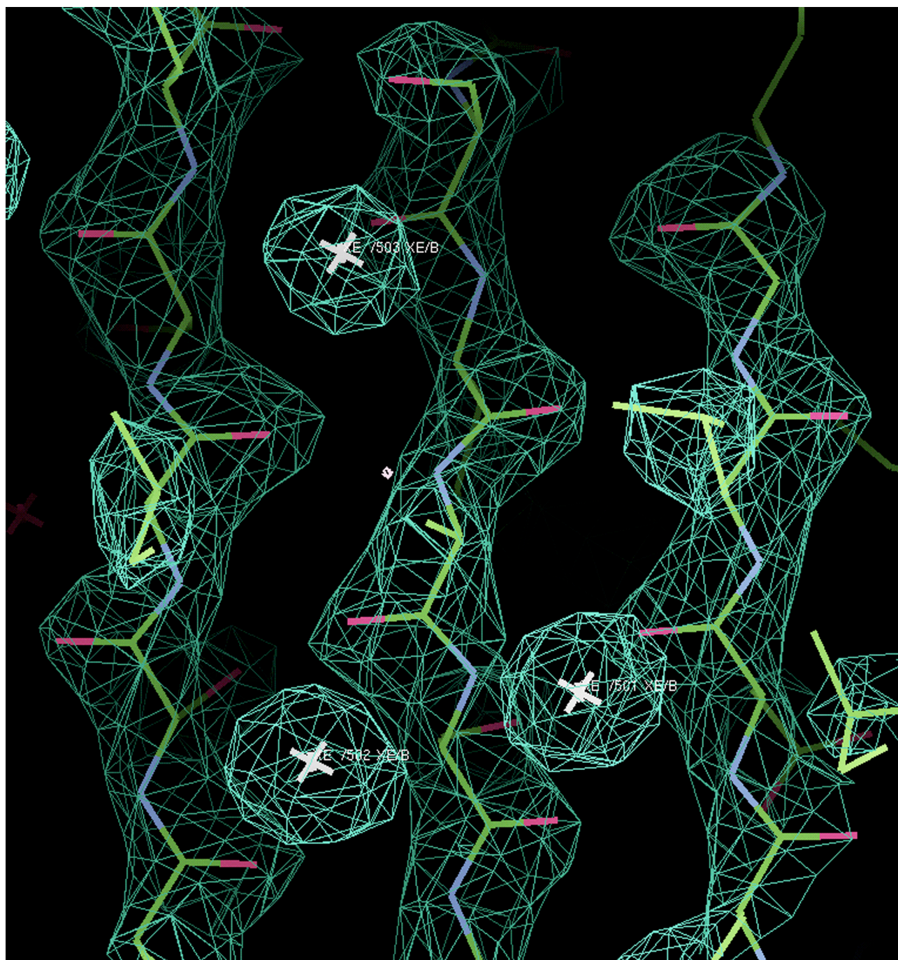
S4 Fig Three xenon sites lining the periphery of the hydrophobic \beta -barrel domain. The 2Fo-Fc map is contoured at 2.5 \sigma . Top: site Xe 503B, lower left: Xe 502B and lower right: Xe 501B (see Table S2).
