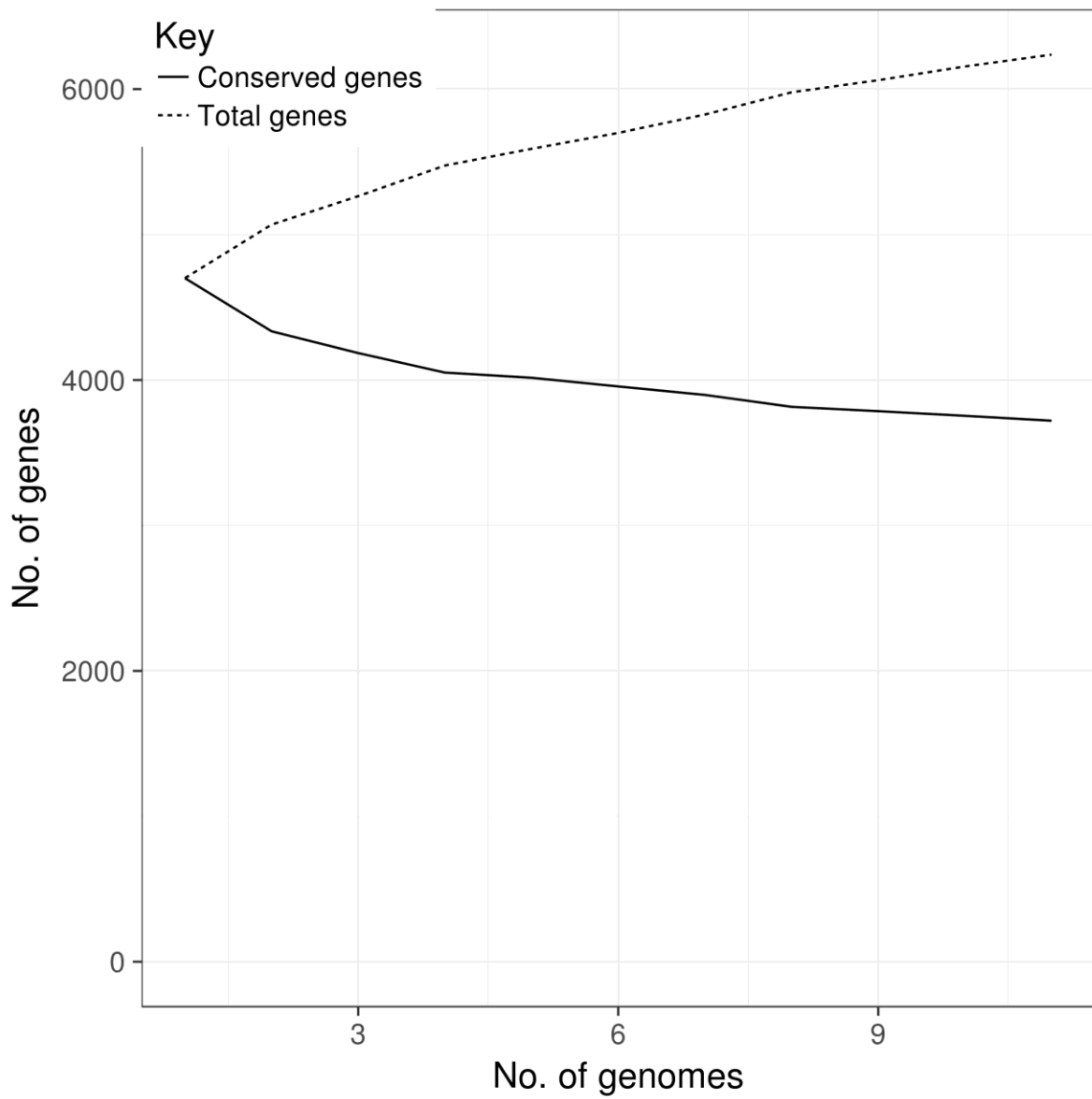
Figure S3. Pangenome accumulation curve. The X- axis indicates the total number of genomes and Y-axis shows the number of genes- conserved vs total gene in S. flexneri pangenome.
