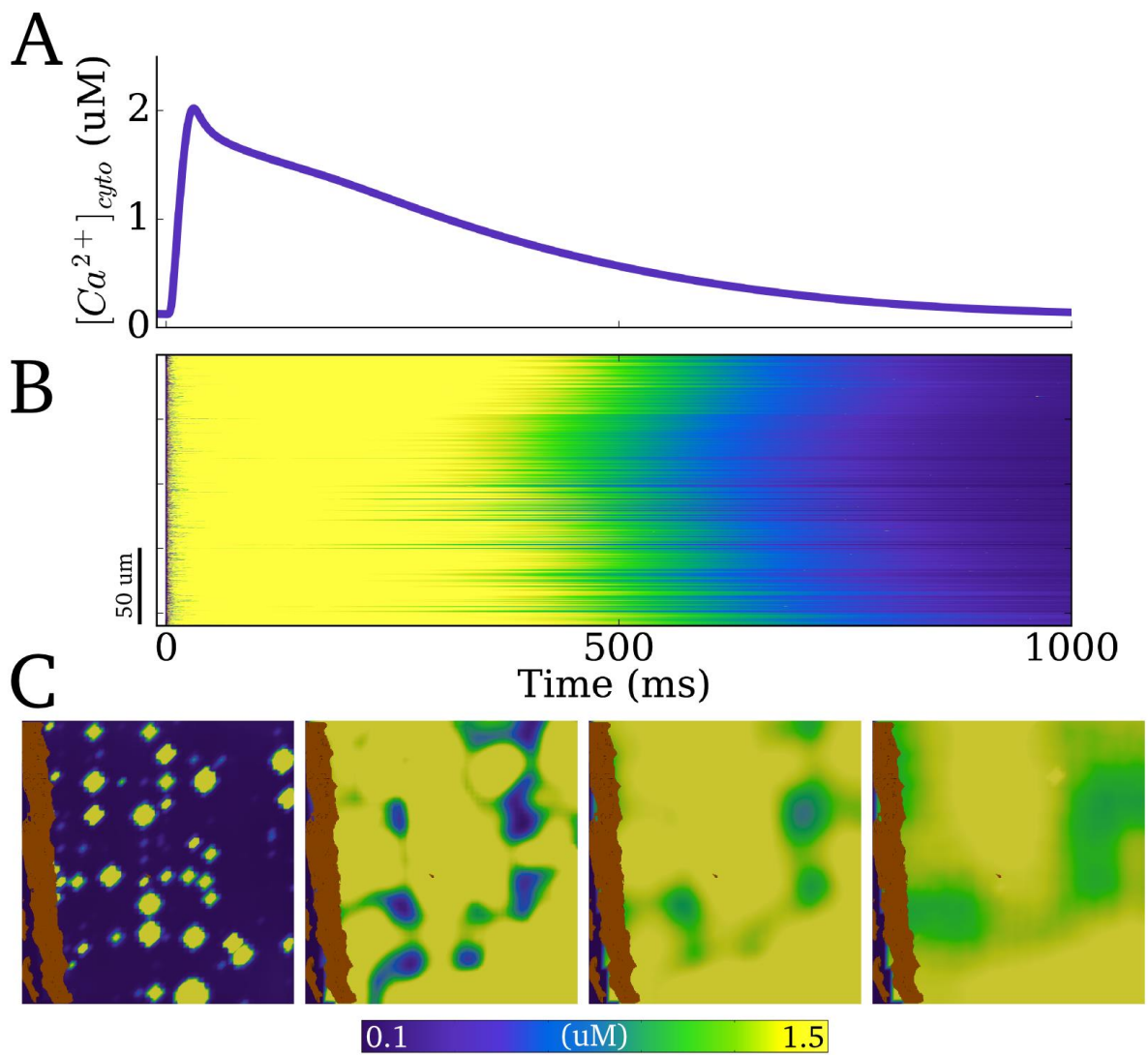
Fig 5: Spatio-temporal dynamics with the Nivala et al 2012 model showing the same snapshots as in Fig 7.
