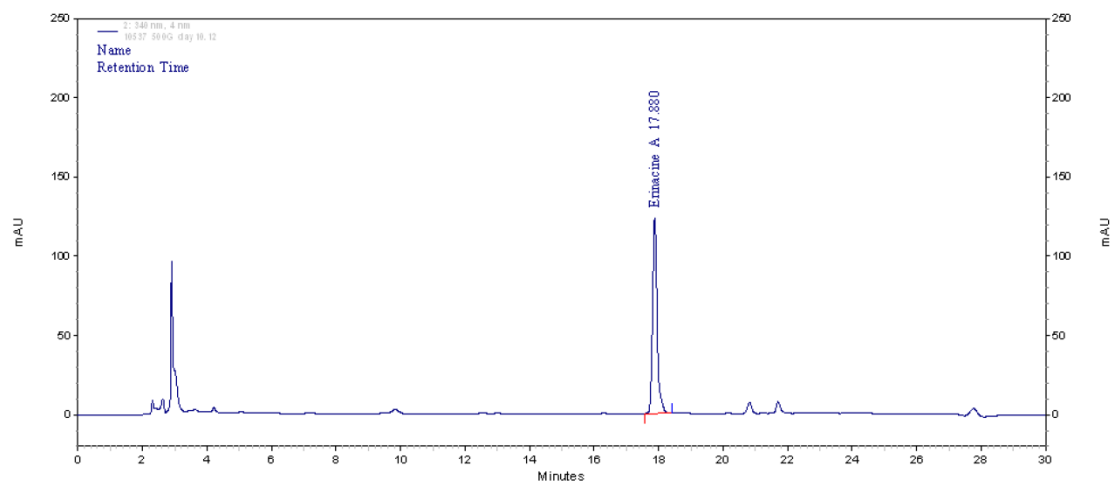
Figure S1. The HPLC chromatograms of the ethanol extract of erinacine A-enriched H. erinaceus mycelium from 20-ton bioreactor (UV detection at 340nm). Retention time of erinacine A is 17.880 min.
