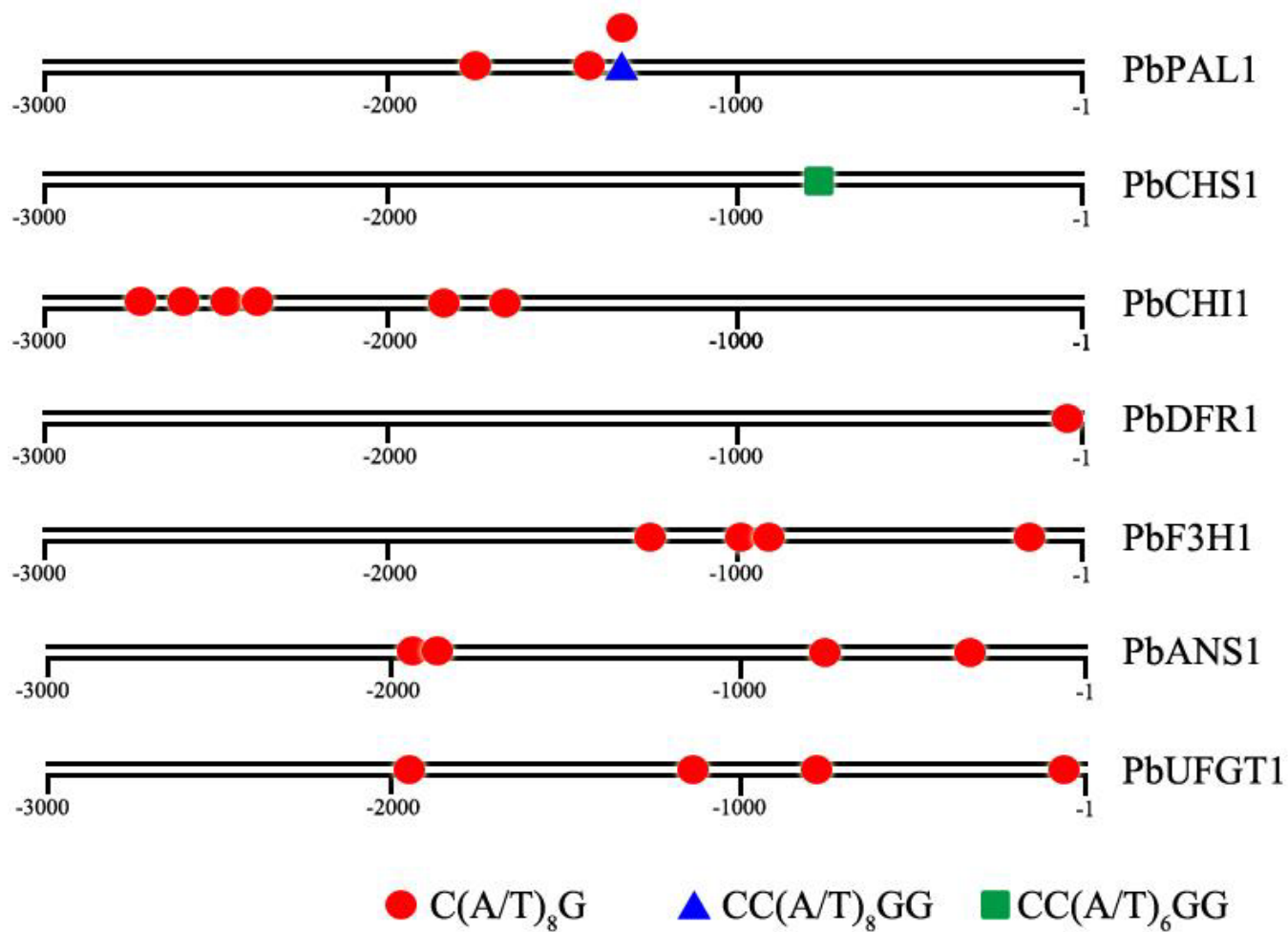
Supplementary figure 8. In silico cis-element prediction of seven anthocyanin biosynthesis genes.
