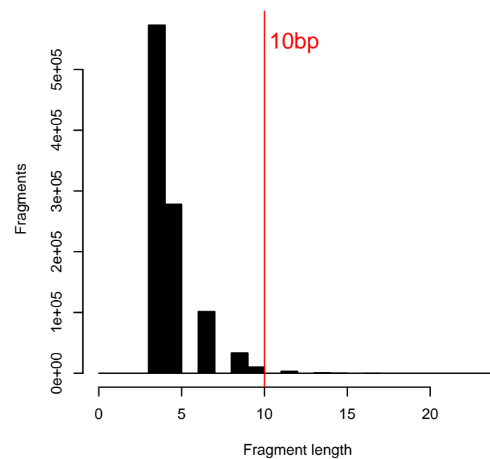
F) N_e = 1e+06 ; generation len = 28
