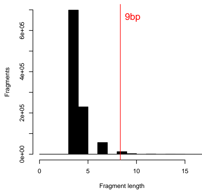
E) N_e = 1e+06 ; generation len = 21
