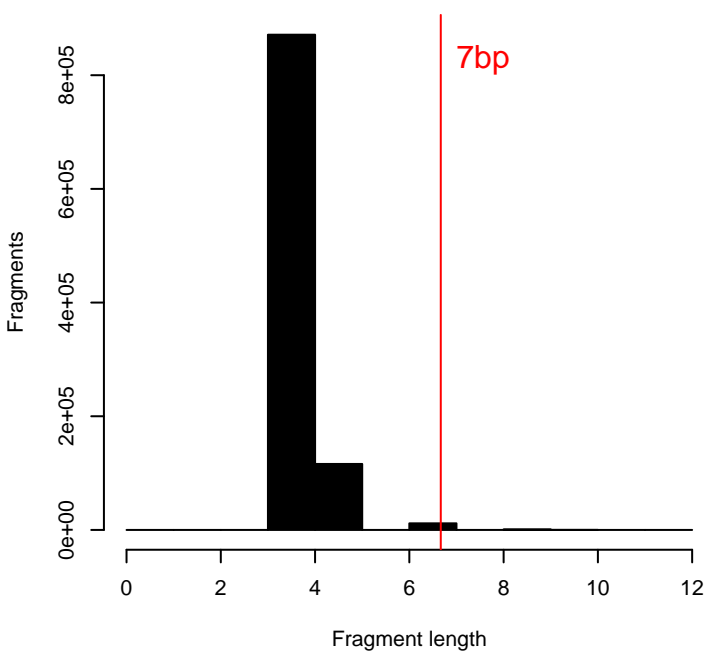
D) N_e = 1e+06 ; generation len = 14
