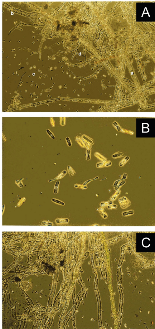
Supplementary Figure 2. Images of phase-contrast microscope of Los Rueldos eukaryotes. (A) [a], [b], filamentous algae; [c] diatoms; [d] cyanobacteria (40X). (B) Detail on the different morphotypes of Los Rueldos diatoms (100X). (C) Image displaying low abundant protozoans (likely from the class Spirotrichea , which includes ciliate protozoans) in open-air water samples (40X).
