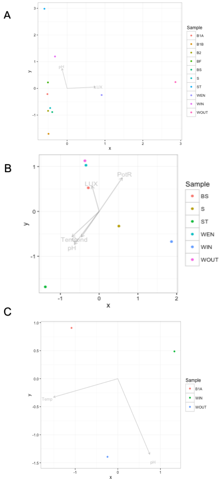
Supplementary Figure 3. Ordination diagrams from canonical correspondence analysis (CCA) of bacterial ( A ), archaeal ( B ) and eukarya ( C ) abundances, and geochemical parameters. Arrows indicate the direction and magnitude of geochemical parameters associated with community structures. Each sample is represented by colored circles according to the collection sites. Abbreviations: PotR, Potential Redox; LUX, Luminance; Temp, Temperature; Cond, Conductivity.
