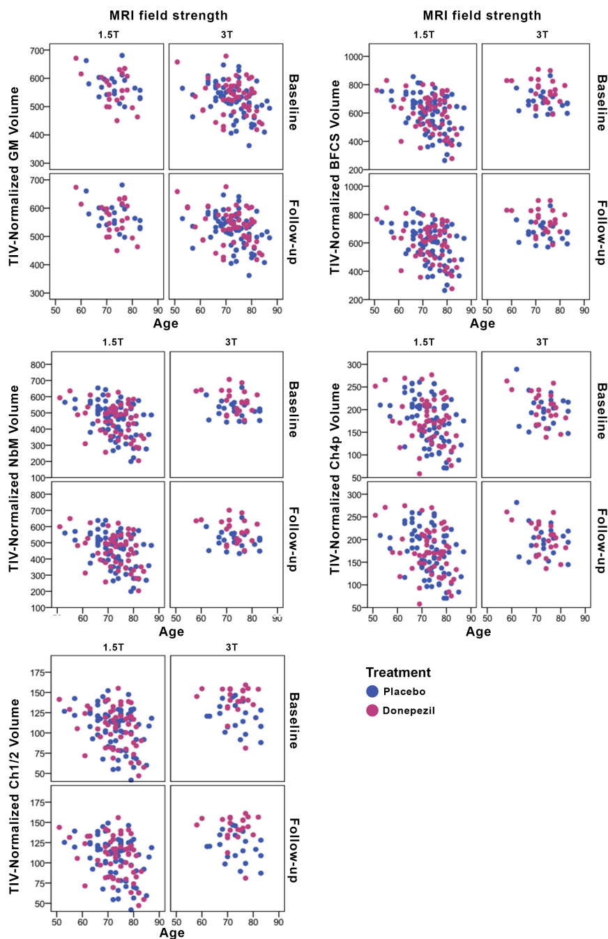
Supplementary Figure 1. Scatter plots describing the distribution of Grey Matter and Basal Forebrain Cholinergic System volumes in each treatment group stratified by MRI field strength at baseline and follow-up scans.
