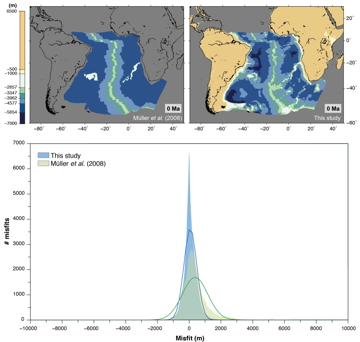
FS01: Top left panel: present day bathymetry as modelled by Müller et al (2008). Top right panel: present day bathymetry as modelled in this study. Bottom panel: Misfits between the two present-day modelled bathymetries and satellite-derived present-day bathymetry. The maps in this figure were generated using the Generic Mapping Tools (Wessel, P. et al. 2013).
