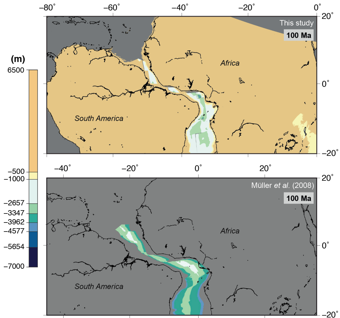
FS02: Differences between modelled paleobathymetry at 100 Ma following our approach (top panel) and that of Müller et al. (2008) (bottom panel). The maps in this figure were generated using the Generic Mapping Tools (Wessel, P. et al. 2013).
