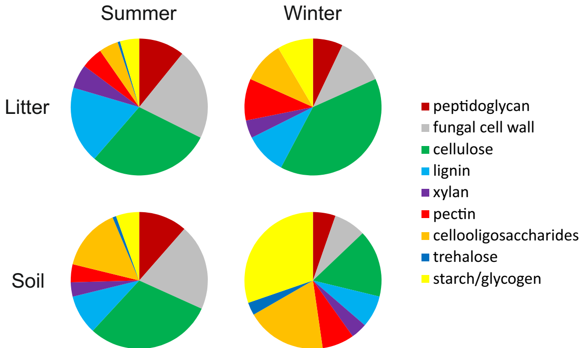
Figure S2.: Functional classification of GH and AA genes with significantly higher expression in summer and in winter within litter and within soil of a Picea abies forest.
