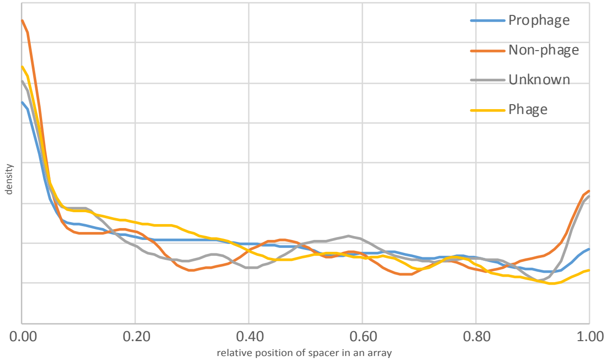
Supplementary Figure 2. Protospacer frequency for relative CRISPR array positions
