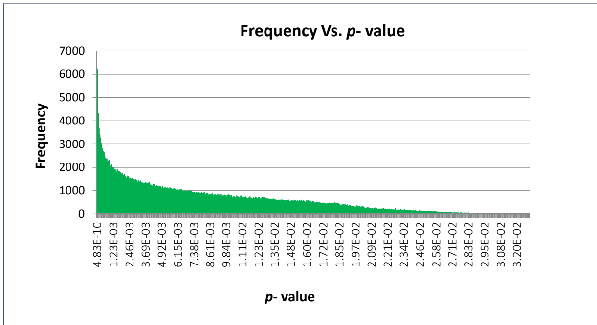
S 2 Fig. The p -value histogram of the top 300000 three-way interactions.
