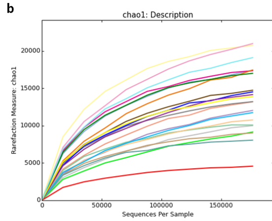
S1 Fig. Rarefaction curves to investigate OTUs were measured by increasing number of sequences in (a) before- and (b) after- metagenome experiments. In the plot, chao1 index was employed to measure alpha diversity in observed OTUs.
