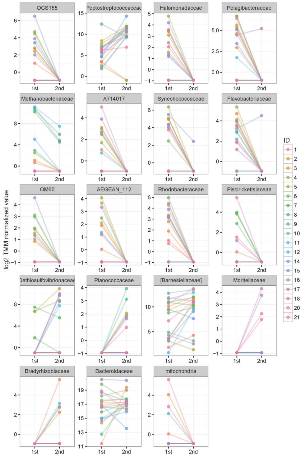
S9 Fig. Line-plots of the 19 significantly detected family-level OTUs.
