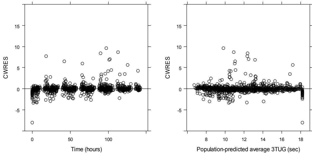
Supplementary Figure S3. Conditional weighted residuals (CWRES) versus time (h) and population predicted 3TUG (sec).
