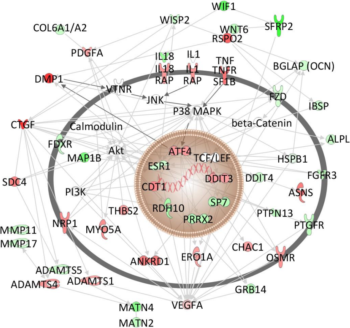
Comprehensive network of putative pathways differentially regulated at pH 7.8 versus 7.4. Upregulated genes (red symbols), down-regulated genes (green symbols), and insignificantly regulated genes (white symbols) were arranged according to a global Ingenuity Pathway Analysis.
