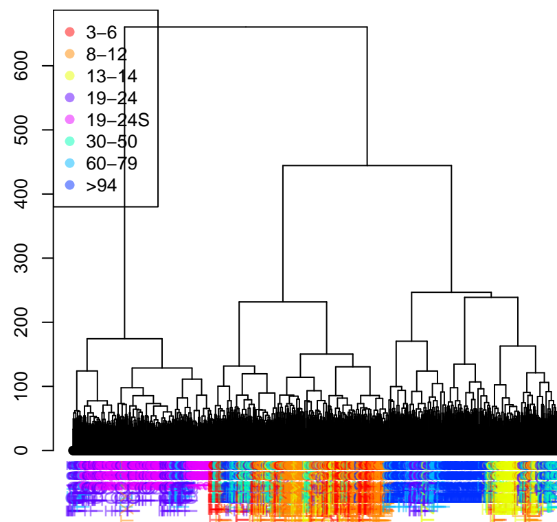
B: dendrogram
