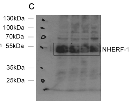
10% SDS-PAGE Gel
