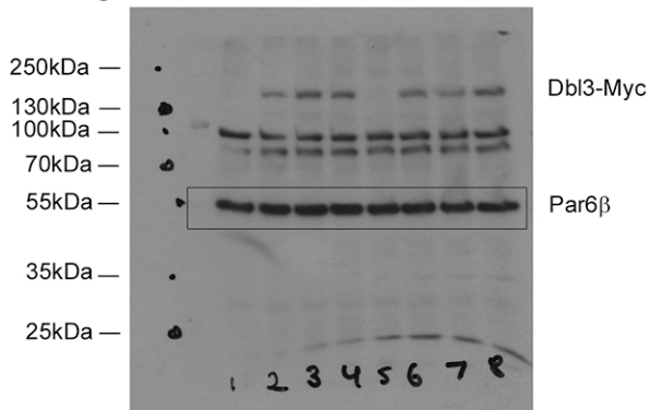
10% SDS-PAGE Gel
