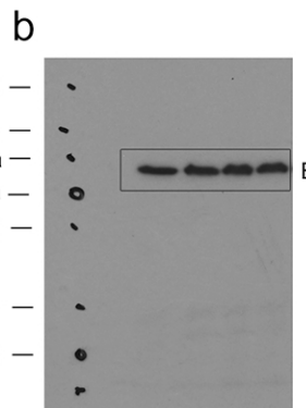
10% SDS-PAGE Gel
