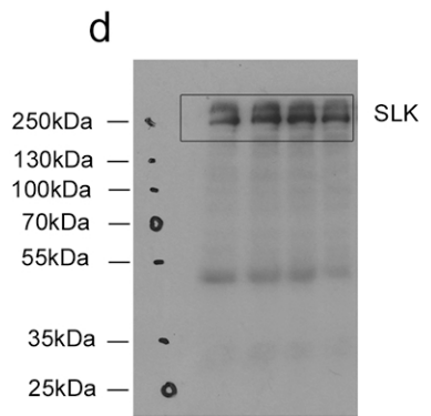
10% SDS-PAGE Gel
